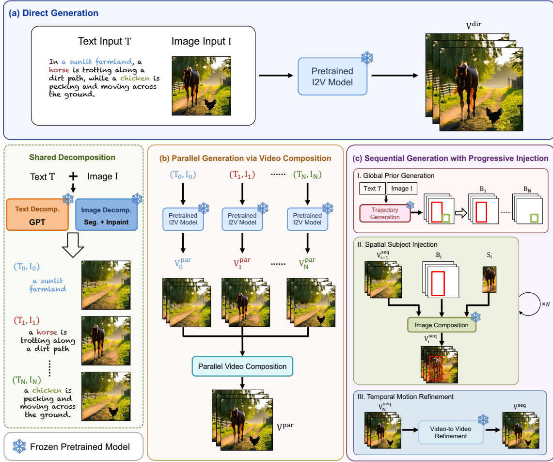
Figure 2: Overview of the compared training-free paradigms for multi-subject image-to-video generation. We compare three strategies: (a) direct generation , which uses the original image and prompt in a single call to a frozen I2V model; (b) parallel generation via video composition , which independently generates decomposed background and subject videos and subsequently composes them; and (c) sequential generation with progressive injection , which inserts subjects one by one into an evolving video. For the decomposed paradigms in (b) and (c), the input prompt T and image I are decomposed into a background pair (T_0, I_0) and subject-specific pairs (T_i, I_i)_{i=1}^N . In (c), stages I, II, and III denote global prior generation, spatial subject injection, and temporal motion refinement, respectively.
