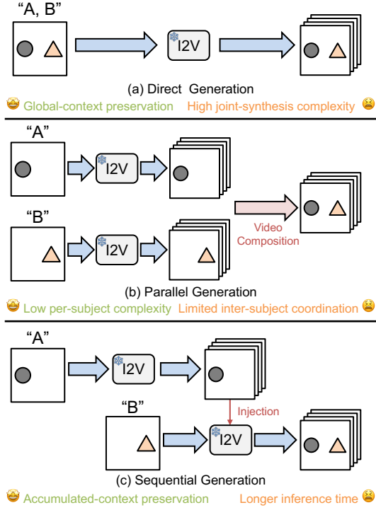
Figure 1: Illustration of three training-free strategies for multi-subject image-to-video generation. Direct generation synthesizes all subjects jointly in one pass; parallel generation independently generates subject-level videos and merges them post hoc; sequential generation injects subjects one by one while conditioning on previously generated video context. The pretrained image-to-video (I2V) models remain frozen across all methods. For simplicity, the decomposition of the input multi-subject image and text prompt is omitted in (b) and (c).
