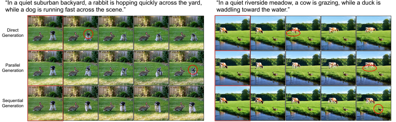
Figure 3: Qualitative comparison of the three paradigms for multi-subject I2V generation. All paradigms use the same pretrained I2VGen-XL [31] backbone. Columns in each block display the 1st, 3rd, 7th, 11th, and 15th frames of the generated videos. The input image I is highlighted with a red box, and the text prompt T is shown above each block. Representative unnatural details are highlighted with red circles.
