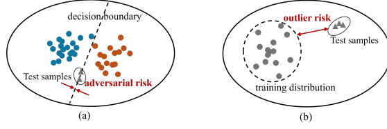
Fig. 1: Illustration of adversarial and outlier risks.
