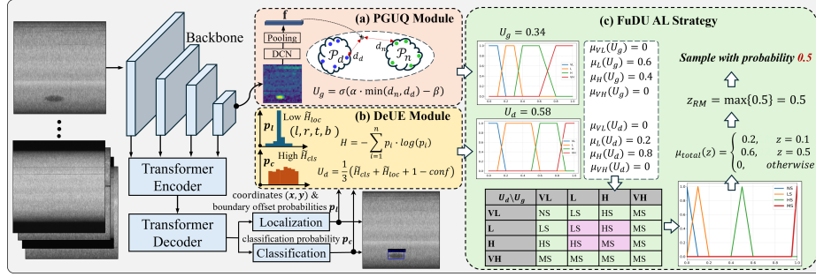
Fig. 3: Overview of the proposed FuDU framework.
