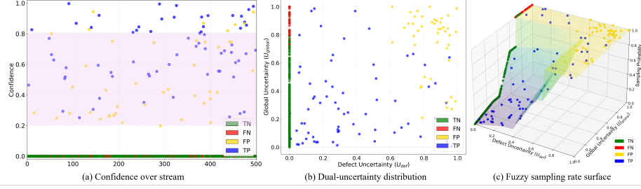
Fig. 2: Comparison of different uncertainty perspectives and sampling strategies on 500 fuel rod images. (a) Image distribution and sampling strategy based on confidence; (b) The image distribution in the dual-uncertainty space; (c) Sampling probability surface based on our FuDU strategy.
