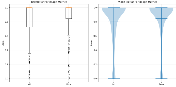
Fig. 7. Distribution of per-image IoU and Dice scores using box and violin plots.
