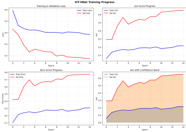
Fig. 10. Training and validation loss, IoU, and Dice over the training epochs.
