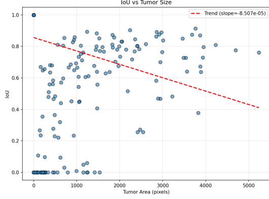
Fig. 6. IoU versus tumor area with a linear trend line.
