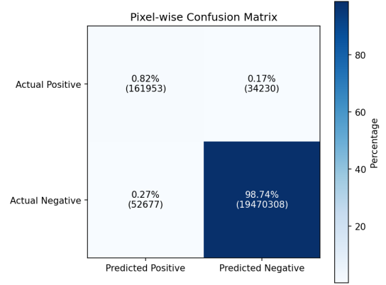
Fig. 4. Pixel-wise confusion matrix heatmap of the proposed model.
