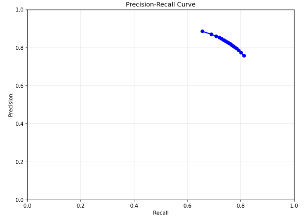
Fig. 5. Precision-Recall curve of the proposed model.
