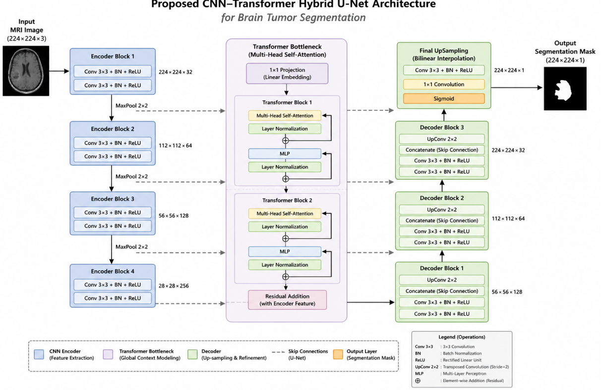
Fig. 2. Proposed ViT-UNet architecture. The encoder extracts hierarchical features, the ViT bottleneck captures global context, and the decoder reconstructs the segmentation map using skip connections.
