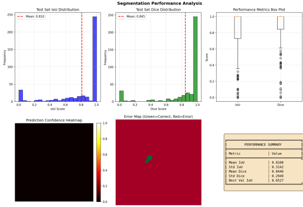
Fig. 3. Performance analysis summary showing various metrics and their distributions.
