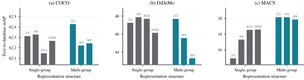
Figure 8: Ablation of single-group and multi-group representation structures. Multi-group contrastive learning consistently improves retrieval performance across different datasets, demonstrating that separating representation capacity into multiple semantic groups provides a more effective basis for adaptive token activation.
