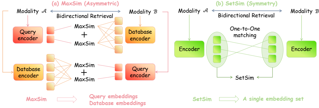
Figure 2: Comparison between MaxSim and SetSim for bidirectional multimodal retrieval. (a) MaxSim defines a directed comparison, leading the two retrieval directions to use role-specific query/database configurations. (b) SetSim performs symmetric one-to-one matching between embedding sets, allowing each modality to use a single embedding set for both retrieval directions.
