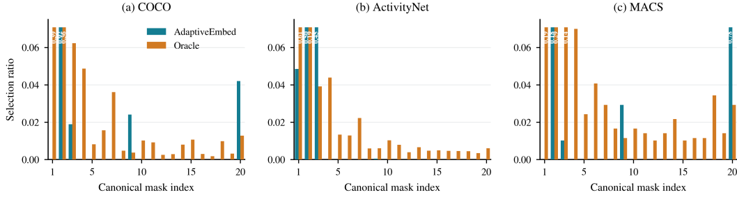
Figure 10: Oracle and AdaptiveEmbed selection distributions on COCO, ActivityNet, and MACS. Each configuration is represented as a binary mask over the eight candidate tokens indicating which are activated; the valid group prefixes yield 20 canonical masks in total. The oracle exhaustively evaluates all 20 masks per sample, whereas AdaptiveEmbed approximates the optimal allocation through its hierarchical policy.
