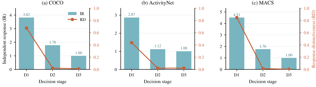
Figure 9: Decision complexity analysis of the hierarchical adaptive policy. The bars show the average number of independent responses required at each decision stage, while the curves indicate the remaining response distinctiveness after each stage. Early decisions provide coarse capacity separation, allowing later stages to operate on a reduced candidate space.
