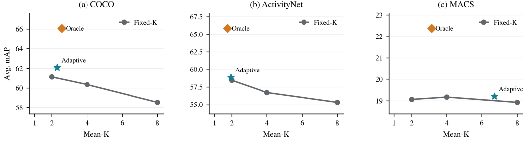
Figure 7: Retrieval utility versus representation cost under adaptive and fixed-capacity allocation, all using the same MGCL-trained representation.
