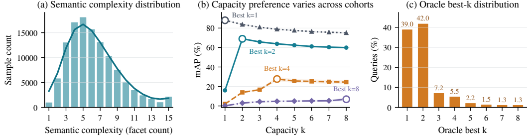
Figure 1: Motivation for sample-adaptive multi-vector representation in multimodal retrieval. (a) Multimodal samples exhibit diverse content characteristics. (b) Samples grouped by oracle-optimal k show different capacity–performance trends, motivating sample-adaptive allocation. (c) Oracle-preferred capacities are distributed across the available range, indicating substantial sample-level variation in representation demand. Results are visualized on COCO.
