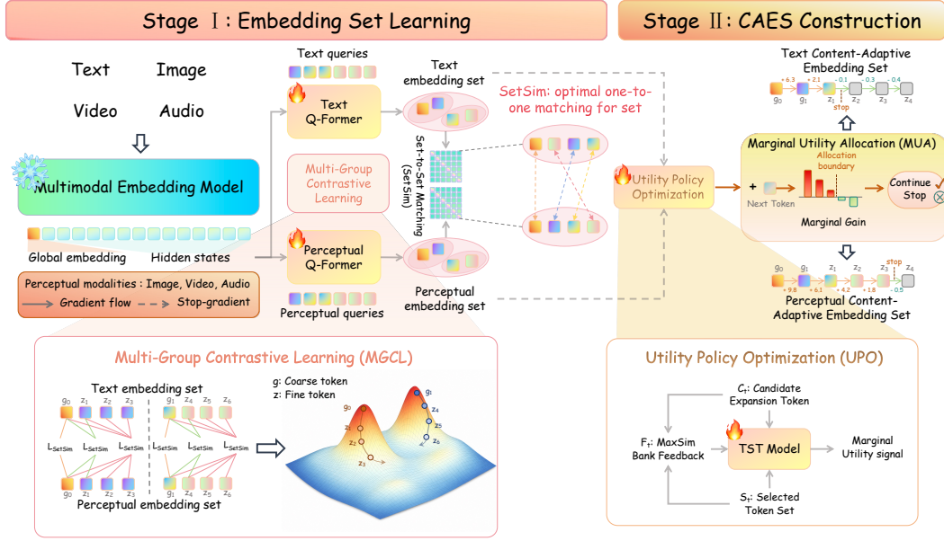
Figure 3: Overview of AdaptiveEmbed. The framework first learns a structured multi-vector embedding set through Multi-Group Contrastive Learning (MGCL), and then constructs a sample-specific content-adaptive embedding set (CAES) using a Token Selection Transformer (TST) trained with Utility Policy Optimization (UPO) and a Marginal Utility Allocation (MUA) strategy.
