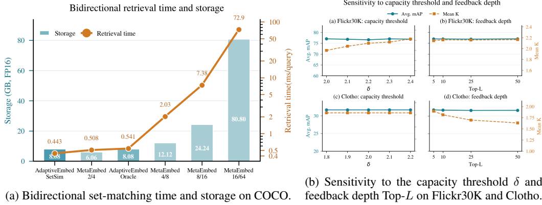
Figure 5: Efficiency and parameter sensitivity analysis of AdaptiveEmbed.
