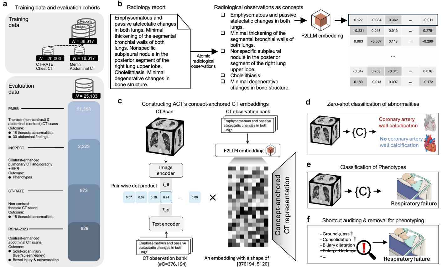
Figure 1: ACT links report-derived observations to prediction and audit. a , Training used chest CT from 20,000 CT-RATE patients and abdominal CT from 18,317 Merlin patients. PMBB, INSPECT, held-out CT-RATE and RSNA-2023 were reserved for evaluation. b , Reports were decomposed into 376,194 atomic radiological observations and embedded with F2LLM. c , For each CT, ACT's native image-text similarities weighted the corresponding F2LLM observation embeddings to yield ACT's normalized 5,120-dimensional concept-anchored CT representation. d-f , ACT's native model supported zero-shot abnormality annotation ( d ), whereas ACT's concept-anchored CT representation supported EHR phenotype classification ( e ) as well as probe-observation audit and observation-bank restriction ( f ).
