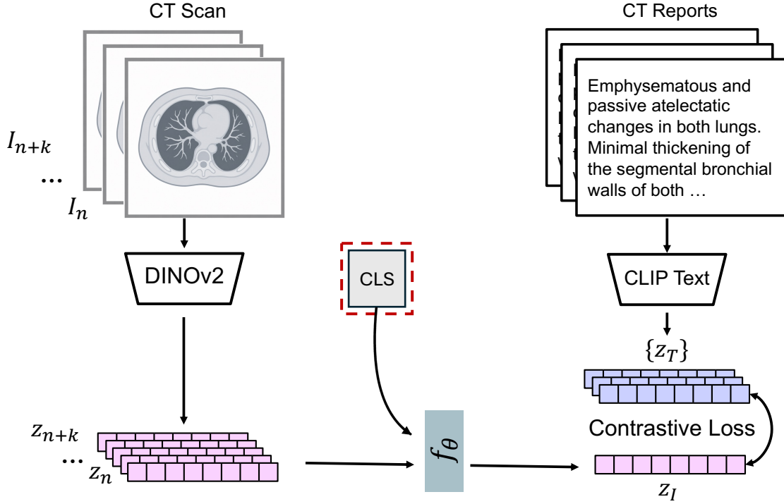
Supplementary Fig. 1: Contrastive pretraining of ACT’s native 3D volume-report model. Each CT volume is resized and padded to 160 \times 224 \times 224 (slices \times height \times width) and represented as a sequence of axial slices. A DINOv2 ViT-B image encoder embeds each slice independently. The Transformer aggregator f_\theta fuses a learnable classification (CLS) token and the slice embeddings into the volume embedding z_I . In parallel, a CLIP-style causal text Transformer encodes the paired radiology impression into z_T . A symmetric contrastive objective aligns z_I and z_T during pretraining on 72,640 paired scan-report rows from 38,317 patients.
