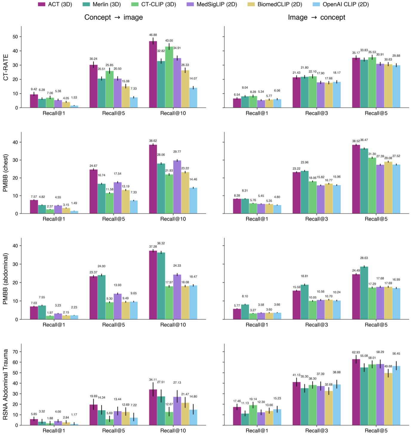
Supplementary Fig. 2: Cross-modal concept retrieval with ACT's native 3D model. Rows show CT-RATE, chest PMBB, abdominal PMBB and RSNA-2023, from top to bottom, for ACT's native model and five baselines. The left column shows concept → image pooled Recall@1/5/10 in 64-candidate pools containing one positive and 63 negative volumes, macro-averaged over findings. Random floors are 1.6%, 7.8% and 15.6%, respectively. The right column shows image → concept Recall@1/3/5 after per-finding z -scoring, averaged over scans with at least one positive finding ( n = 2,226, 8,843, 11,646 and 265, respectively). Bars are full-sample point estimates. Error bars show percentile 95% CIs from 1,000 patient-clustered bootstrap resamples shared across models.
