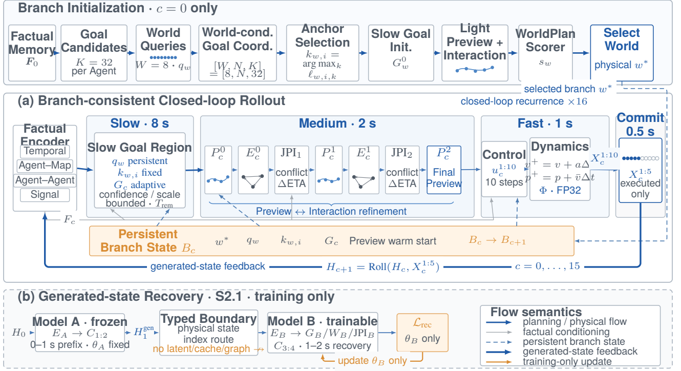
Figure 1. Architecture of Hi-FLoop. At initialization, eight scene-level Worlds propose joint future branches and the scorer selects one physical World whose identity persists through all 16 commits. The recurrent core updates an 8-s Goal, alternates two rounds of 2-s Preview–Interaction refinement, decodes 1-s Control, and writes only the executed 0.5-s prefix back to factual history. The S2.1 path uses a frozen A→B recovery cascade: its typed boundary transfers physical state and causal context, but no latent state, cache, or gradient graph.
