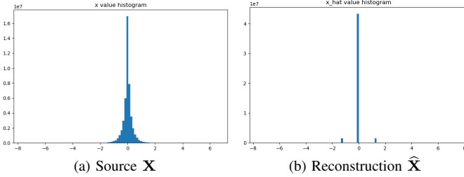
Fig. 5. Value distributions of the primary visual-token representation before and after NNC compression. The reconstruction concentrates on a smaller set of discrete values, consistent with strong quantization.
