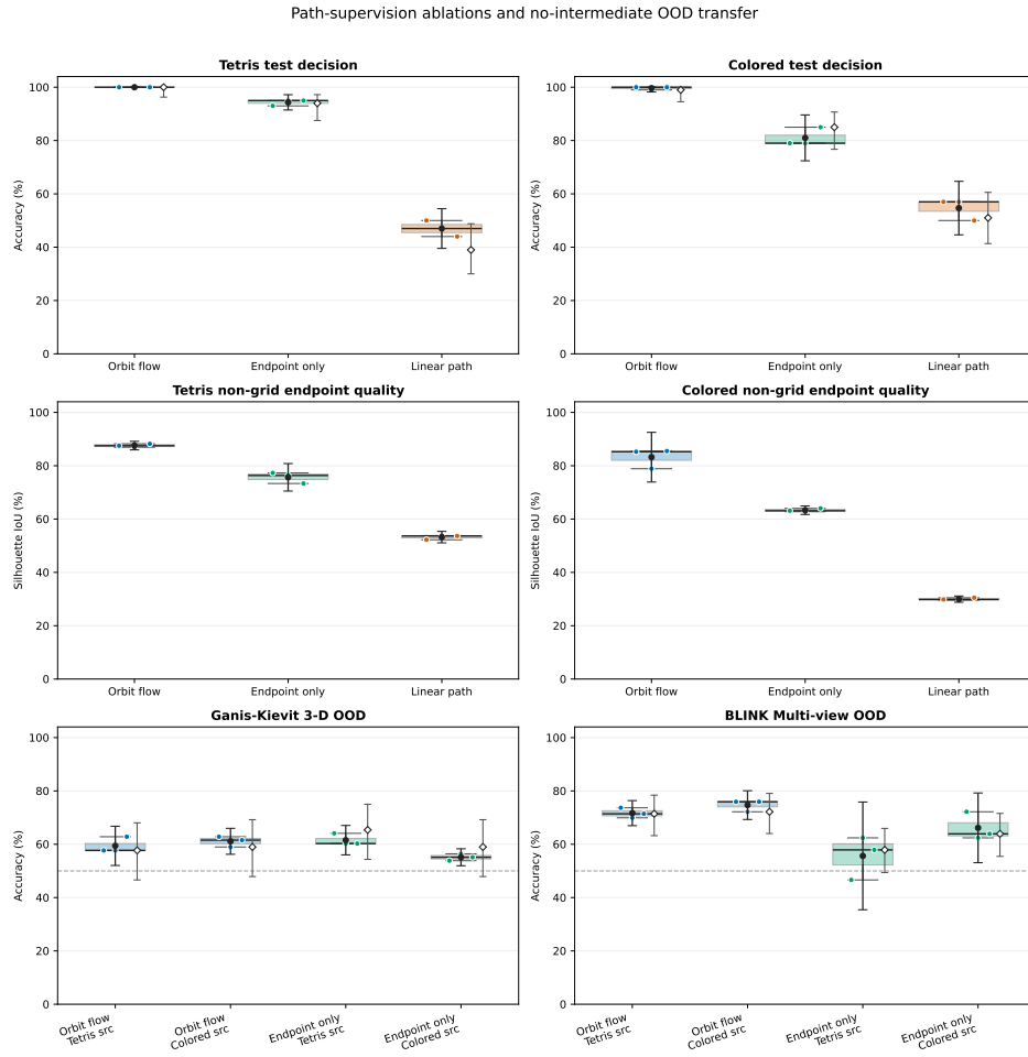
Figure 6: Matched path ablations and no-intermediate OOD controls. Boxes span three training seeds and retain all raw points; black circles and bars denote seed means and two-sided Student- t 95% intervals. Open diamonds on accuracy panels denote seed-ensemble decisions with Wilson intervals over items.
