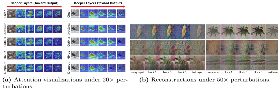
Fig. 5: Robustness under extreme perturbations. (a) Only Aether progressively suppresses perturbations—becoming increasingly similar to the clean image as layers approach the output—yielding class-consistent latents. Conventional augmentations such as CutMix, Mixup, and Dropout retain residual artifacts. (b) Late-layer feature inversions show that Aether preserves semantic information even under heavy corruption, producing reconstructions highly similar to the clean image with only minor perturbations.
