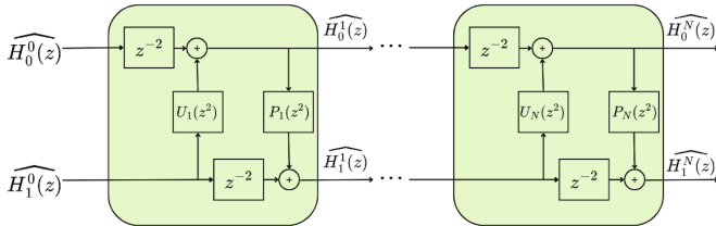
Fig. 2. Lifting Scheme Structure for the analysis part of the filter bank, with lifting functions U_k(z^2) and P_k(z^2) .
