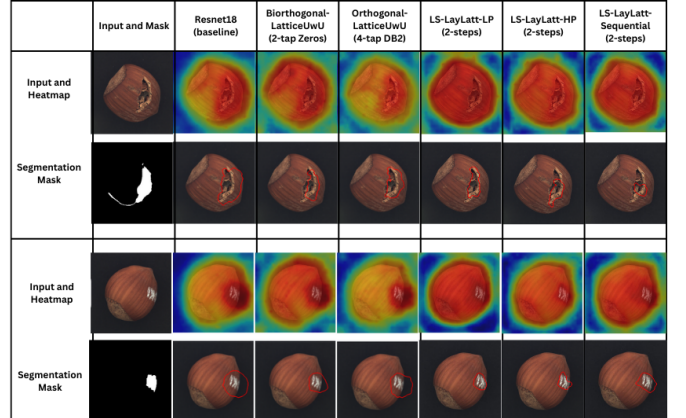
Fig. 3. Segmentation and heatmaps generated by the CFLOW-AD method on the MVTec AD hazelnut dataset using a pretrained proposed and baseline methods with ResNet-18 backbone.
