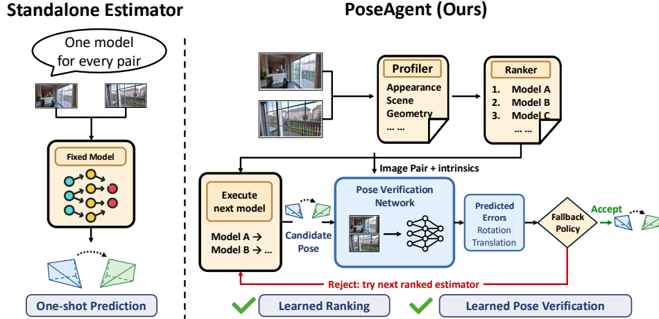
Figure 1: We propose PoseAgent , an agentic framework that adaptively ranks and executes pose estimators and verifies pose estimation with orchestration. Our framework is a meta-learner and improves a set of standalone pose estimators.
