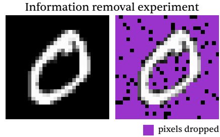
Figure 13: MNIST sparsification protocol. Models are trained on complete images. At evaluation, pixels with value v \leq 0.5 are progressively removed, while pixels with value v > 0.5 are always retained.
