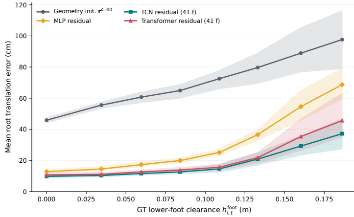
(a) Root error as a function of lower-foot clearance above the pitch.
