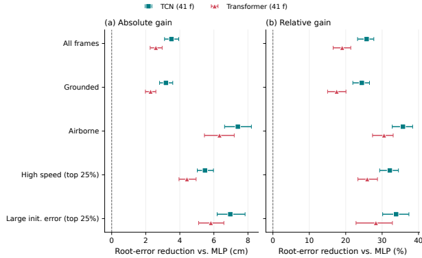
Figure 6. Relative improvement of temporal models over the frame-wise MLP across different motion regimes.
