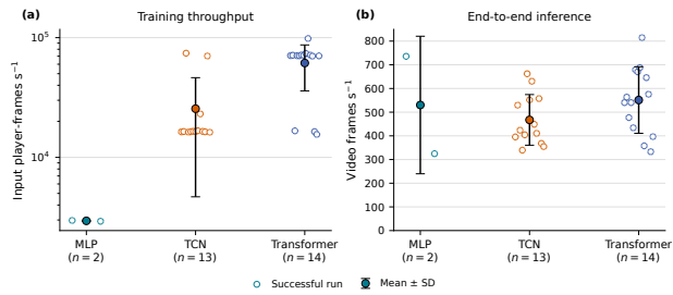
Figure 12. Computational throughput of the MLP, TCN, and Transformer architectures on an NVIDIA L40S GPU. (a) Training throughput in input player-frames per second. (b) End-to-end inference throughput in video frames per second. Each hollow marker represents one successfully completed run, while filled markers and error bars indicate the mean and standard deviation across runs. Training throughput counts the player-frame tokens processed by the optimization loop, including overlapping temporal windows.
