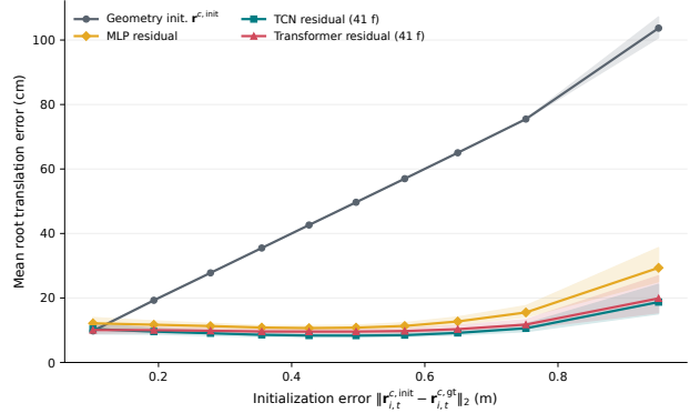
Figure 4. Root error as a function of the geometry-based initialization error. Temporal residual refinement remains substantially more stable than the raw geometric estimate as initialization quality deteriorates.
