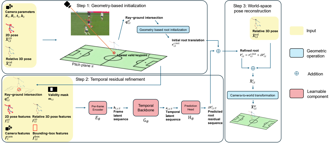
Figure 3. Overview of the proposed Field Converter method. First, a geometry-based initialization estimates the player root from the calibrated camera, the relative 3D pose, and a ray-ground intersection. Second, a temporal model predicts a residual correction using pose, image, camera, and geometric cues. Finally, the refined root anchors the relative skeleton in camera coordinates before transformation to the common world coordinate system.
