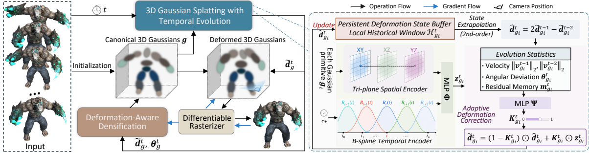
Figure 4: The overall architecture of EvoGS . Instead of the standard modeling for Gaussian deformation using observation MLP, we propose the temporal deformation evolution mechanism to temporally learn Gaussian deformation field across time. Furthermore, we develop the deformation-aware densification strategy, which initializes newly created Gaussians based on the updated deformation and prevents densification in regions with high deformation uncertainty.
