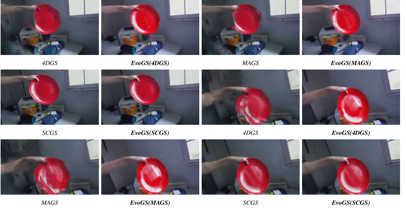
Figure 8: Qualitative comparison on the NeRF-DS dataset. The baselines (4DGS and MAGS) produce severely distorted object contours, where the plate boundary and arm silhouette are noticeably warped. The EvoGS-augmented variants ( EvoGS(4DGS) and EvoGS(MAGS) ) preserve much more stable geometry and sharper outlines, demonstrating that the proposed temporal deformation evolution modeling consistently stabilizes geometry and appearance across diverse dynamic Gaussian frameworks.
