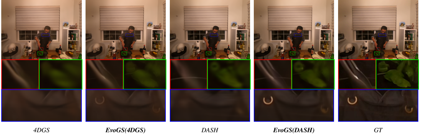
Figure 6: Visual comparisons on Neu3D dataset. The zoomed views reveal that the baselines produce over-smoothed structures on the metal strap (red box), the spinach leaves (green box), and the ring details on the clothes (blue box). Incorporating our temporal deformation evolution modeling substantially sharpens these structures, restores richer local contrast, and yields more faithful fine-scale geometry and appearance across both backbones.
