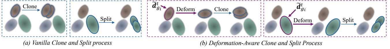
Figure 5: Illustration of the proposed deformation-aware clone-and-split process. Compared with the vanilla strategy, our method integrates deformation cues to initialize new Gaussians with motion-adaptive geometry, leading to more consistent and stable updates across frames.
