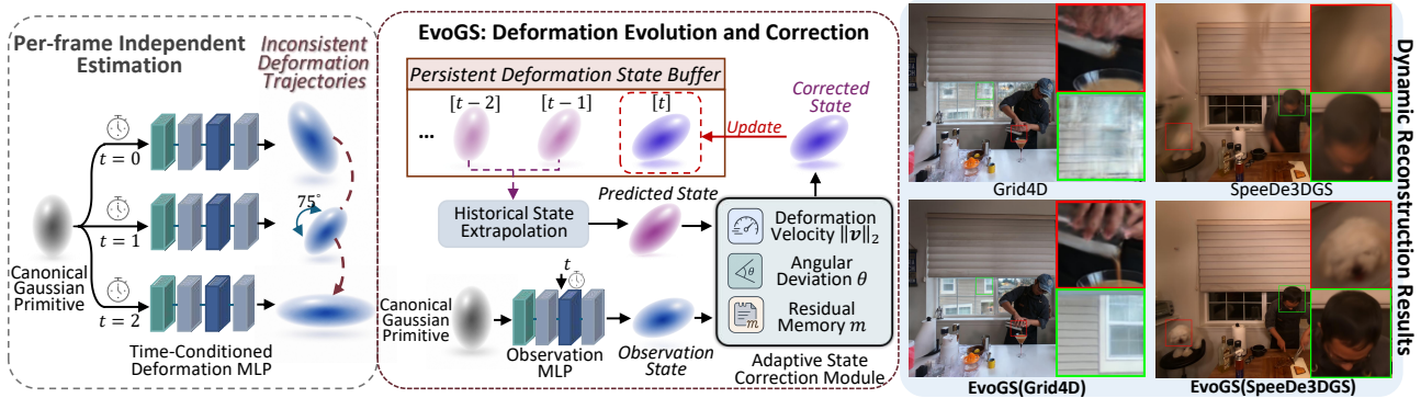
Figure 1: Existing dynamic 3DGS methods often estimate deformations separately at each timestamp, which can lead to temporal artifacts and unstable reconstruction. EvoGS maintains persistent deformation states and performs evolution-based correction. The qualitative results show that integrating EvoGS improves different dynamic Gaussian backbones, producing sharper details and better-preserved geometry.
