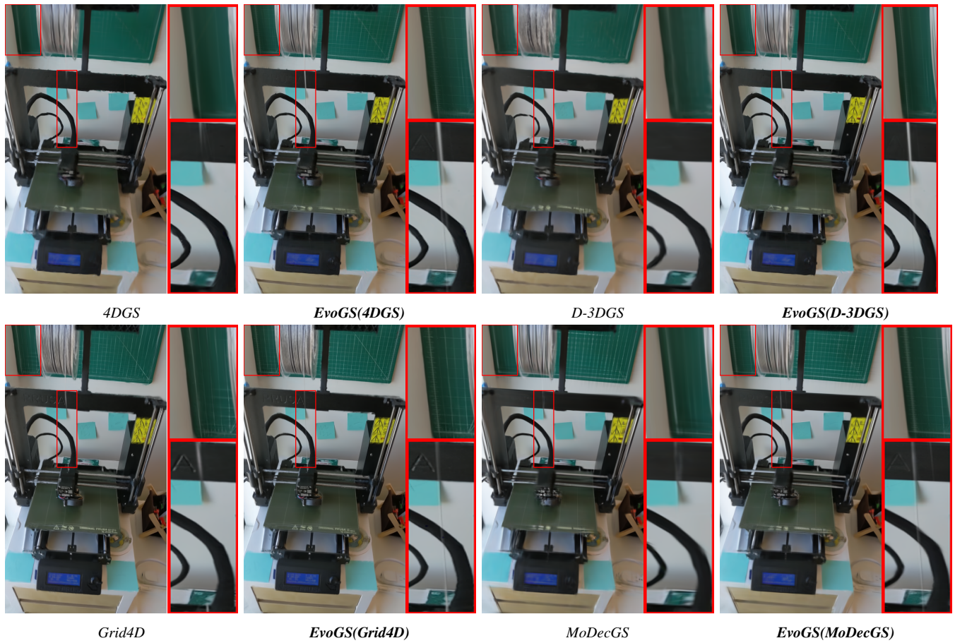
Figure 9: Qualitative comparisons on a complex scene with thin structures and sharp planar geometry (3D printer scene in HyperNeRF dataset). The zoomed crops highlight that our EvoGS variants built upon various baselines enhance boundary localization and structural fidelity: vertical edges on the cutting mat become straighter and less wavy, the black cable and metallic frame exhibit fewer double edges and ringing artifacts, and small high-contrast details are better preserved, demonstrating consistent improvements across compared baselines.
