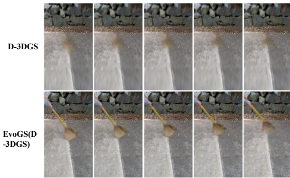
Figure 10: Visualizations of novel views rendered with the same camera pose across consecutive timesteps on the HyperNeRF (vrig) dataset. Specifically, the baseline D-3DGS fails to represent the moving broom. In contrast, EvoGS achieves good reconstructions of the moving broom and background structures across frames.
