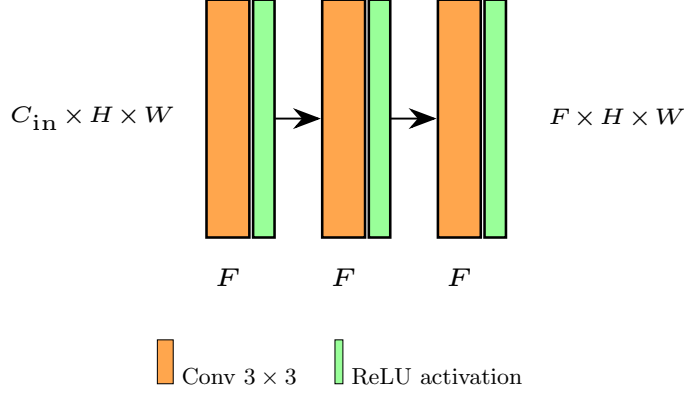
Fig. 2 Feature-extraction block used across DeepBM3D ( \phi_\theta , \psi_\theta^{\text{img}} , and \psi_\theta^{\text{dct}} ). The module is three consecutive Conv 3×3 + ReLU layers with reflect padding, thus preserving the spatial size ( H \times W ). For the image-level extractor \phi_\theta , the channel sizes are C_{\text{in}}=2 (noisy image and noise map) and F=32 ( light ) / F=64 ( heavy ). For the patch-level extractors \psi_\theta^{\text{img}} and \psi_\theta^{\text{dct}} , C_{\text{in}}=N candidates with N=C+1 , and F=Nm with m=4 ( light ) / m=8 ( heavy ).
