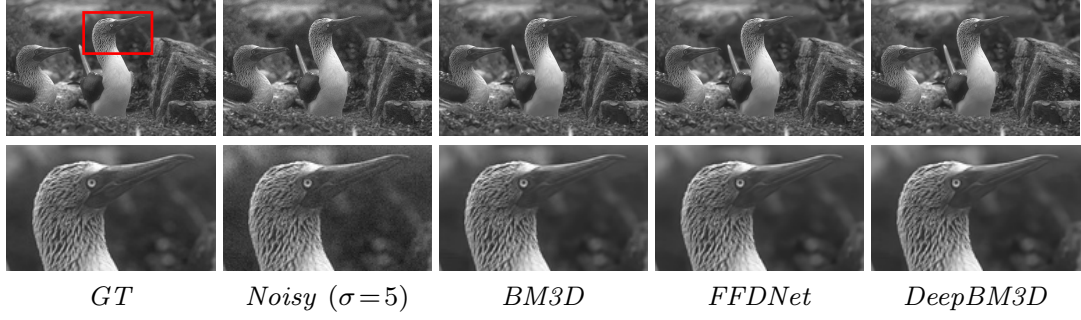
Fig. 4 Qualitative comparison on BSD100 at \sigma=5 . Top: full images (GT annotated with zoom region). Bottom: identical zoomed region across methods.
