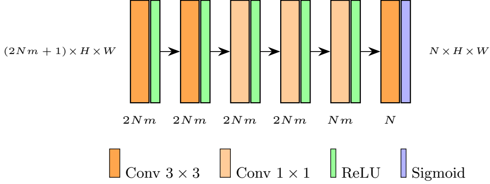
Fig. 3 Wiener weights estimation network ( \omega_{\theta}^{(1)} and \omega_{\theta}^{(2)} ). The model combines Conv 3 \times 3 , Conv 1 \times 1 , and nonlinear activations to map features of size (2Nm+1) \times H \times W to Wiener weights of size N \times H \times W . All convolutions use reflect padding. Here, N denotes the number of grouped patches and m the internal capacity multiplier. In the light configuration, m=4 ; in the heavy configuration, m=8 .
