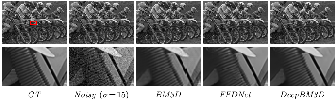
Fig. 5 Qualitative comparison on Kodak at \sigma=15 . Top: full images (GT annotated with zoom region). Bottom: identical zoomed region across methods.
