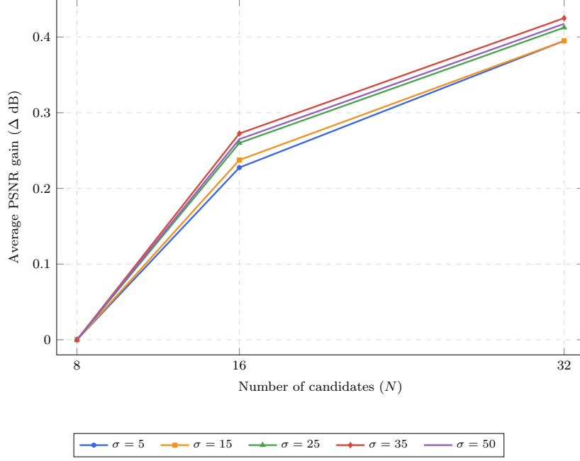
Fig. 10 Effect of the number of candidates. Average PSNR gain ( \Delta dB) achieved by varying the number of candidates ( N ) in the light flexible DeepBM3D configuration, relative to the lightest setting with N=8 , across different noise levels.
