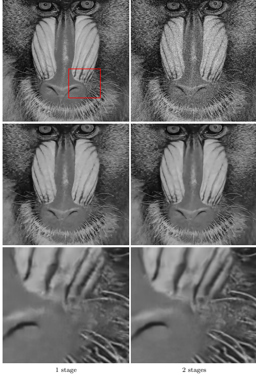
Fig. 9 Comparison of the one- and two-stage variants of DeepBM3D on Set14 at \sigma = 35 . The two-stage model refines the first-stage output, yielding sharper and cleaner details in the zoomed region.
