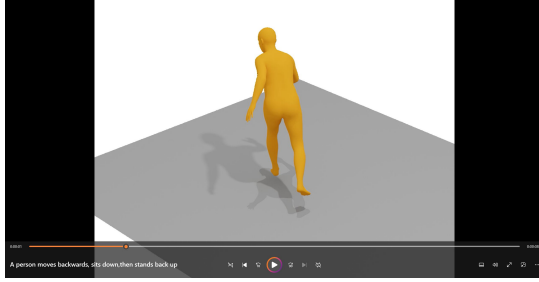
Fig. 12: Video sample.
