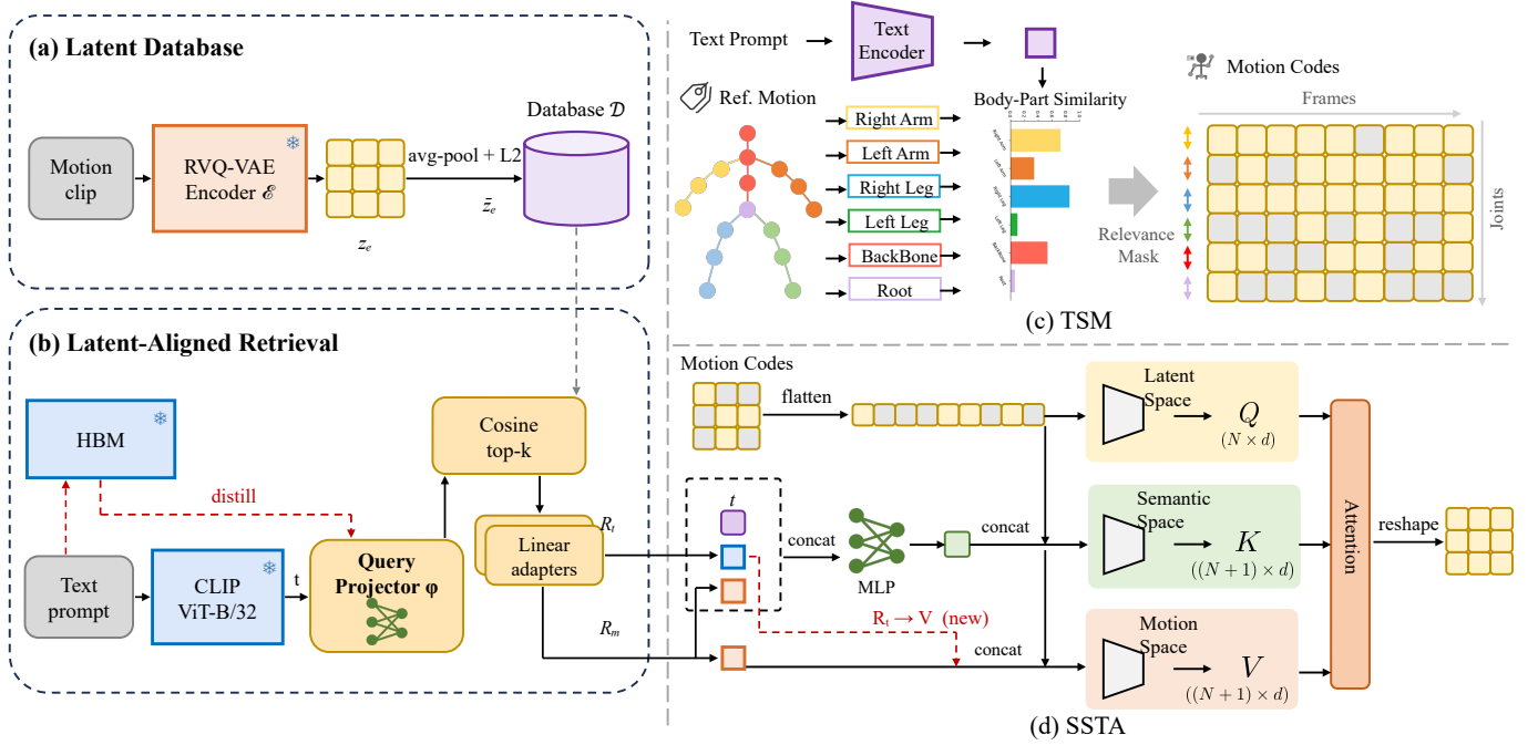
Fig. 3: Framework of ReMoMask-2. (a) The retrieval database is built offline by the frozen RVQ-VAE encoder \mathcal{E} : each motion becomes a pre-quantisation latent grid, pooled and \ell_2 -normalised into a key. (b) A query projector \phi , distilled from the frozen HBM retriever, maps text into that same key space, so cosine retrieval returns evidence already expressed in the generator’s representation. (c) Topology Structured Masking (TSM) and (d) Semantic Spatial–Temporal Attention (SSTA) are inherited unchanged from ReMoMask, except that R_t may now enter the Value pathway.
