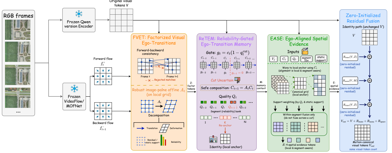
Fig. 2. Overview of EGOsis, a pose-free RGB adapter for UAV video reasoning. FVET factorizes bidirectional flow, ReTEM gates and re-anchors transition memory, and EASE aligns visual evidence to segment anchors. The resulting contexts Z , M , and E update frozen Qwen visual features through zero-initialized residuals without changing the visual-token count.
