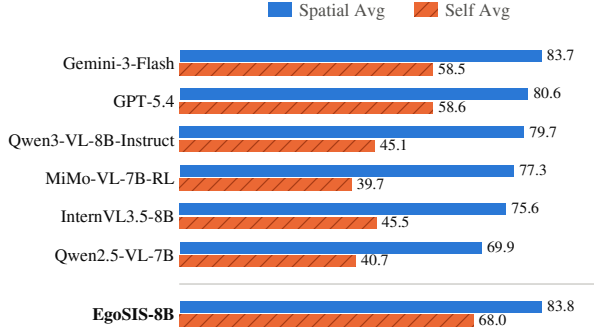
Fig. 3. Question-weighted dimension accuracy using counts reconstructed from Table 1.
