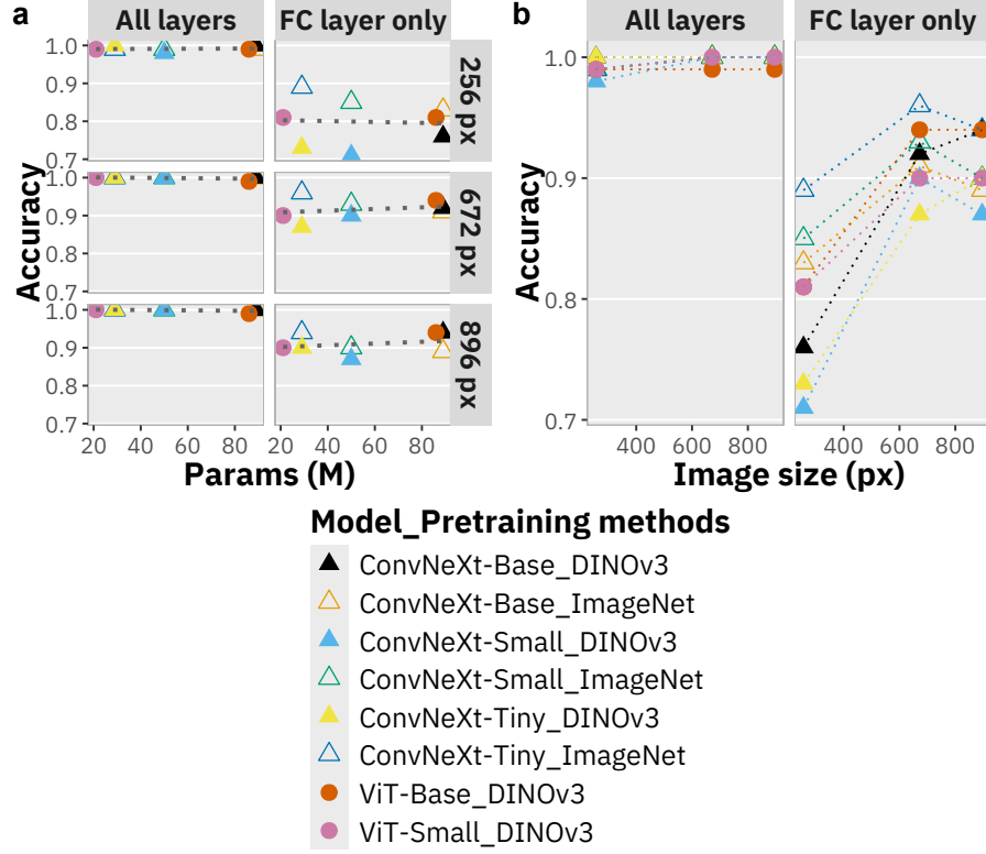
Fig. 3. Accuracy of the 48 models evaluated in this study: (a) Separate panels are shown for each input image size and training strategy, with either all layers or only the FC layer unfrozen. The horizontal axis in each panel represents model size. The dashed lines indicate linear regression fits; (b) Separate panels are shown for the two training strategies, with either all layers or only the FC layer unfrozen. The horizontal axis in each panel represents the input image size.
