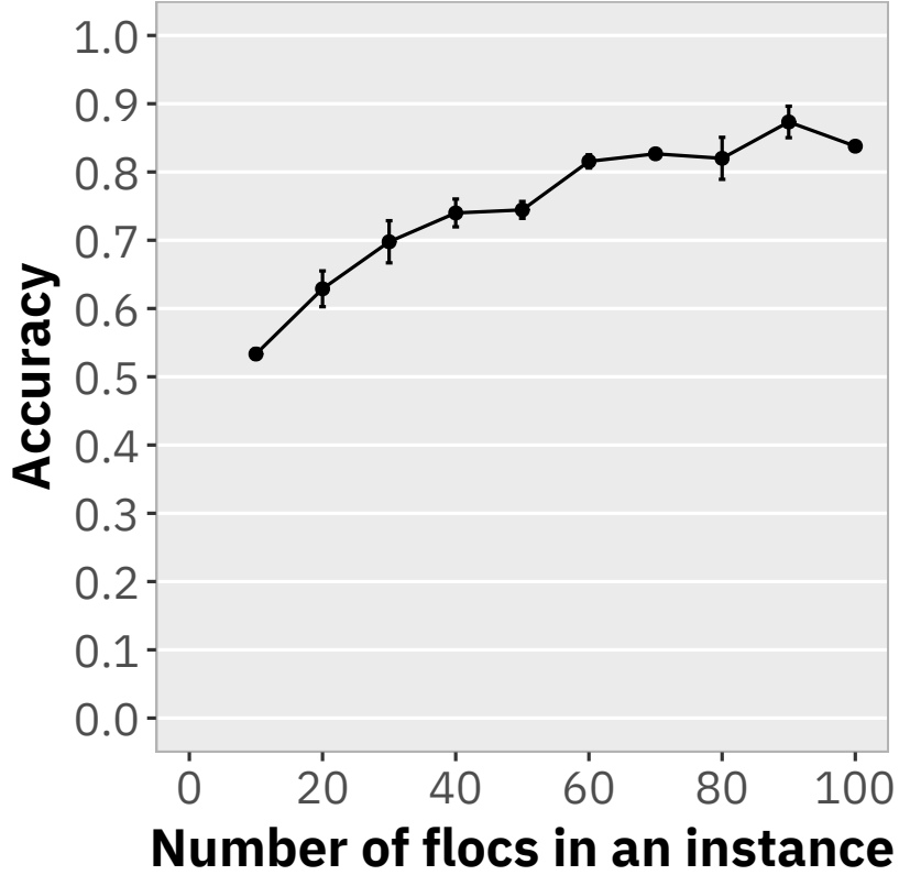
Fig. 6. Relationship between the number of flocs per instance and classification accuracy in benchmark tasks using QIA-derived morphological parameters and machine learning. The error bars indicate the standard error.
