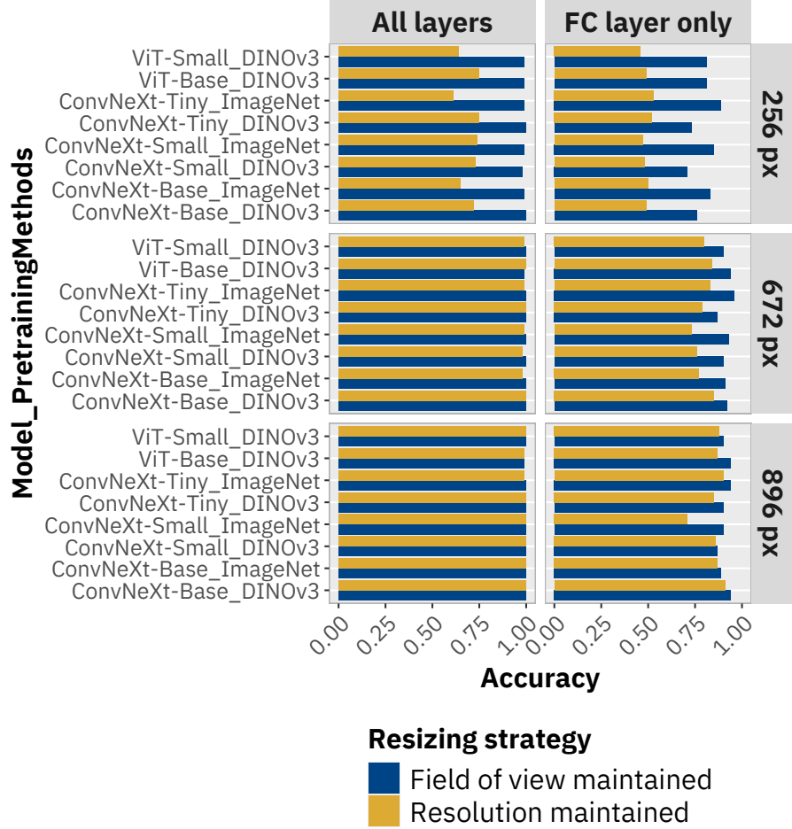
Fig. 5. Comparison of accuracy between resizing strategies that maintain the field of view and resolution. Accuracy obtained from our 96 trained models is shown in separate panels for each image size and training strategy. Bar length represents accuracy. Blue bars indicate results obtained when the field of view was maintained, whereas yellow bars indicate results obtained when the resolution was maintained.
