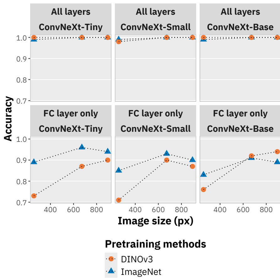
Fig. 4. Differences in accuracy achieved by our ConvNeXt models across pretraining methods.
