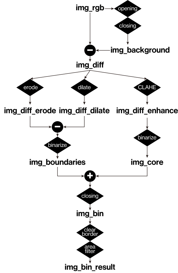
Fig. 2. The binarization procedure for quantitative image analysis
