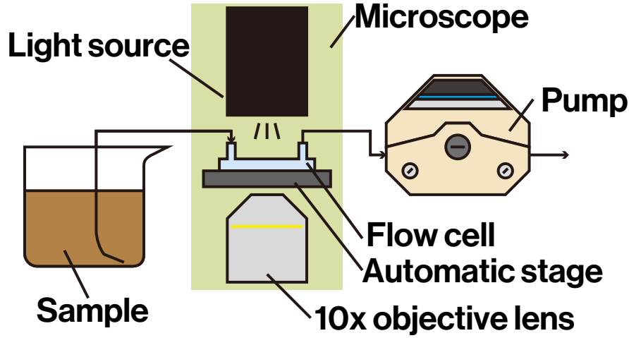
Fig. 1. Structure of a automated imaging system
