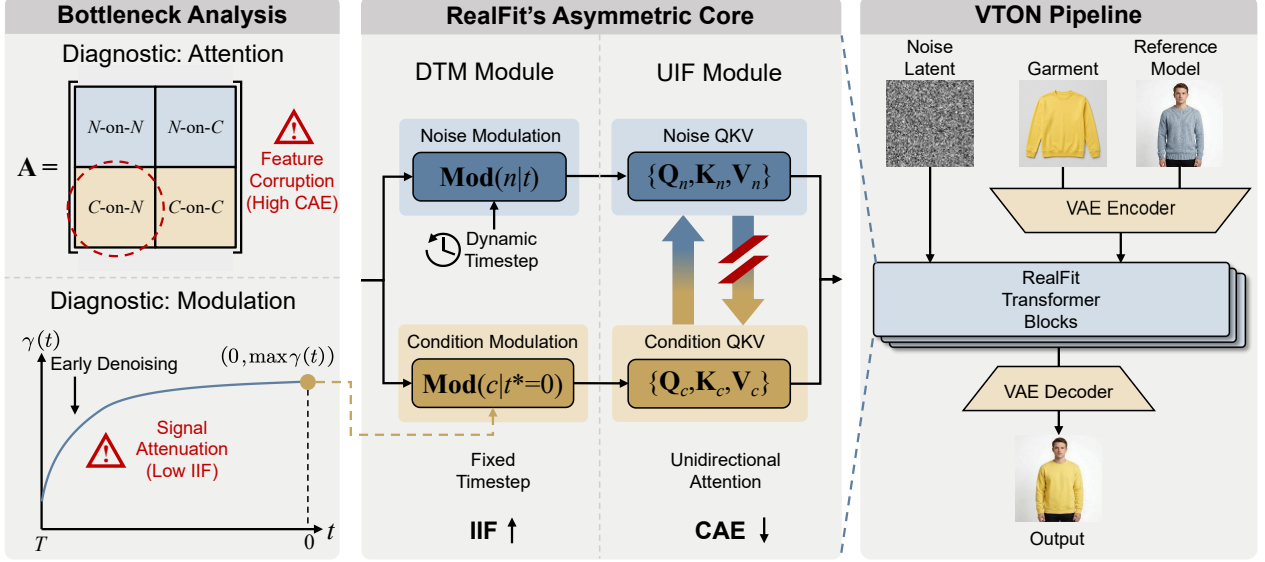
Figure 2 Overview of RealFit. High CAE in attention and low IIF in modulation can create an information bottleneck. RealFit addresses this bottleneck through an asymmetric design that combines UIF and DTM for high-fidelity VTON.
