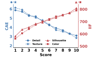
Figure 5 CAE/IIF trends with perceptual fidelity.
