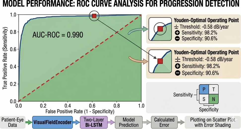
Figure 3: Receiver operating characteristic curve for fast-progressor detection (MD < -1 dB yr ^{-1} ) on the held-out test set. AUC = 0.990 (95% confidence interval by stratified bootstrap: 0.982–0.996). The Youden-optimal operating point (predicted MD threshold = -0.58 dB yr ^{-1} ; sensitivity 98.2%, specificity 90.6%) is marked. AUC, area under the receiver operating characteristic curve; MD, mean deviation.
