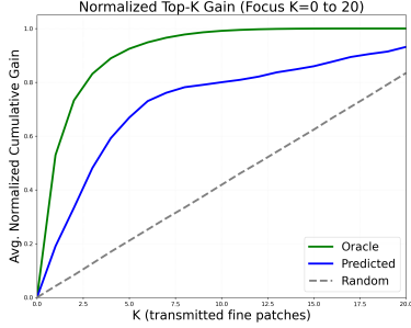
Figure 8. Per-agent Top- K normalized cumulative marginal detection gain ( K \leq 20 ). Ranking patches by our predicted benefit score \beta successfully concentrates the majority of attainable detection gain within a strict low- K budget cap regime, vastly outperforming random allocation.
