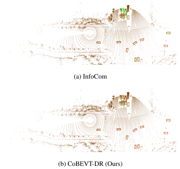
Figure 9. Qualitative comparison. Green: ground truth. Red: detections. (a) InfoCom relies on pure sparsification, discarding unselected regions and missing several vehicles in the upper-right cluster. (b) CoBEVT-DR at a strict 2 KB budget recovers the cluster; the dense coarse floor provides a continuous semantic anchor even for unselected objects.
