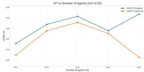
Figure 7. Scaling with number of agents under fixed budgets (OPV2V). AP@0.5 versus non-ego agent count N at a 2.0KB/agent cap for CoBEVT-DR. Dense CoBEVT uses \sim 6.3 MB/agent ( \sim 31.4 MB total network payload at N=5 ), whereas CoBEVT-DR uses \sim 2.0 KB/agent ( \sim 10 KB total at N=5 ).
