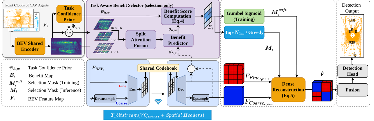
Figure 1. Overview of our Dual-Resolution Budget-Aware Transmission Framework. CAV i extracts BEV features F_i (Sec. 3.1) and computes a pooled task-confidence prior \psi_{h,w} (Sec. 3.2). Guided by \psi_{h,w} , the selector predicts a benefit map B_i to output a soft mask M_i^{soft} for budgeted training via dual ascent (Secs. 3.3 and 3.4), or a deterministic Top- N_{fine} mask M_i for strict inference constraints. The ego vehicle decodes the highly compressed payload (VQ indices and spatial headers) to reconstruct M_i and the dense feature map \hat{F} for fusion (Sec. 3.6). The dashed arrow ( \bar{d}_{h,w} ) denotes the regularized offline supervision target (Sec. 3.5).
