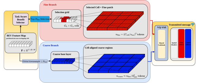
Figure 2. Spatial hierarchy and bitstream composition. The selector sends selected cells as fine patches, while a globally downsampled BEV map provides the dense coarse base layer. Both branches share the VQ-VAE codebook; the bitstream stores spatial headers, fine indices, and coarse indices.
