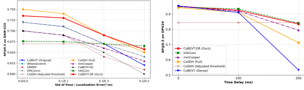
(a) Pose and Localization Error Robustness on DAIR-V2X Dataset (b) Time Delay Robustness on OPV2V
