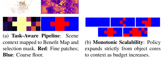
Figure 3. Integrated Scalability Analysis. Visual logic (a) and mask expansion (b) illustrate the learned refinement policy used for fixed and dynamic budget adaptation.
