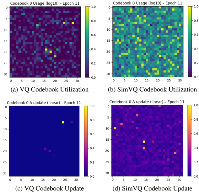
Figure 5. Comparison of codebook dynamics at Epoch 11. (a) and (c) show that standard VQ collapses, with only a few vectors being utilized or updated. (b) and (d) demonstrate that SimVQ maintains a healthy, distributed codebook usage and consistent updates across the entire grid.
