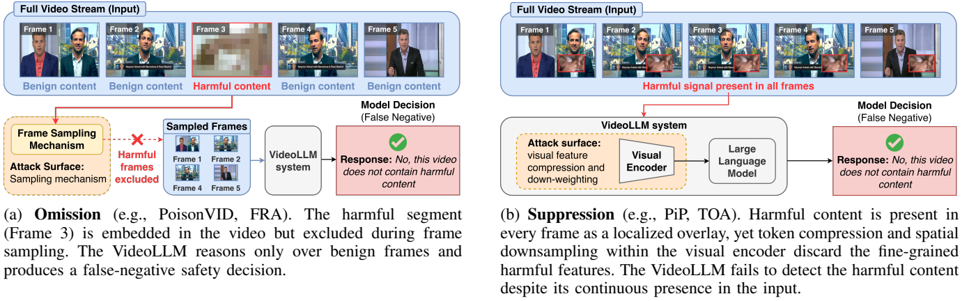
Fig. 1: Two categories of observation-level attacks against VideoLLMs. Both cause false-negative safety decisions, but through different mechanisms. In (a), harmful frames are never sampled. In (b), harmful signals enter all sampled frames but are suppressed during internal processing.
