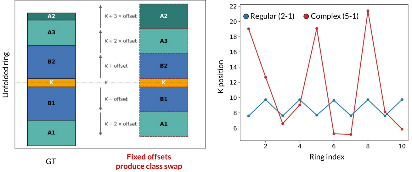
Figure 11: Structural constraints of the fixed SAM4Tun labelling rule. (a) Labelling rule: after K is detected, B segments are placed one step either side of K and A segments at successive multiples of the same fixed offset, in a fixed order, so the template mislabels rings whose segment widths or count differ from the reference. (b) Ground-truth K position versus ring index for one regular (blue, 2-1) and one complex (red, 5-1) tunnel: K jumps from ring to ring, much more on the complex tunnel, which the current one-configuration-per-tunnel setting does not address.
