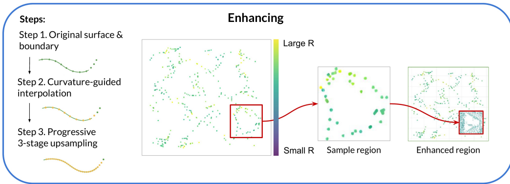
Figure 5: Stage 3: Enhancing. Left: curvature-guided surface and boundary interpolation along the tunnel lining, showing original sampling, curvature-guided insertion, and progressive three-stage upsampling (shown as three sequential upsampling steps). Centre: unfolded 2D depth map after enhancement, where inserted points improve geometric continuity; the red box highlights a local region of interest. Right: zoomed views of the highlighted region, showing added points and pixel-level interpolation.
