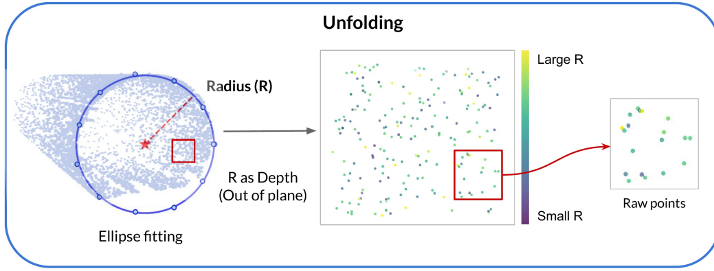
Figure 3: Stage 1: Unfolding. Left: fitted tunnel cross-section used to determine the reference centre and radius for cylindrical unfolding. Centre: 2D panoramic depth map derived from the 3D point cloud. Right: zoomed region of the unfolded map showing radial-distance encoding.
