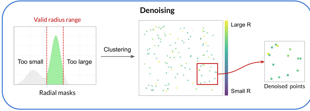
Figure 4: Stage 2: Denoising. Left: radial-distance distribution used to filter points outside the expected tunnel lining surface. Centre: unfolded 2D depth map after filtering, showing the cleaned point distribution. Right: zoomed region of the denoised map.
