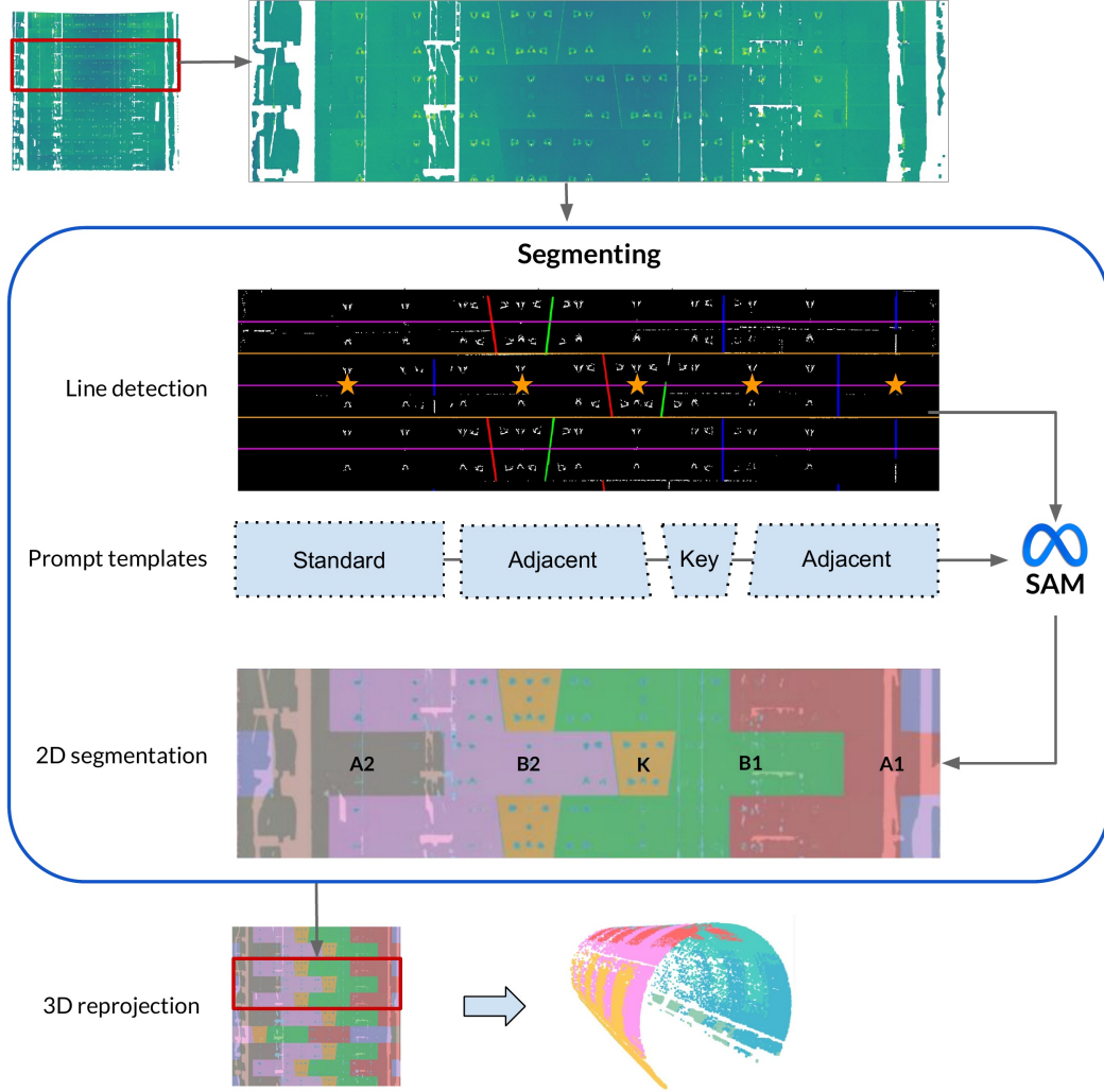
Figure 6: Stage 4: Segmenting. The segmenting stage applies Hough-transform line detection [56] to identify ring boundaries, then constructs template-based prompts and feeds them to SAM [12]. SAM produces 2D segment masks that are reprojected into 3D. K denotes the key segment, B denotes adjacent segments, and A denotes standard segments around the ring.
