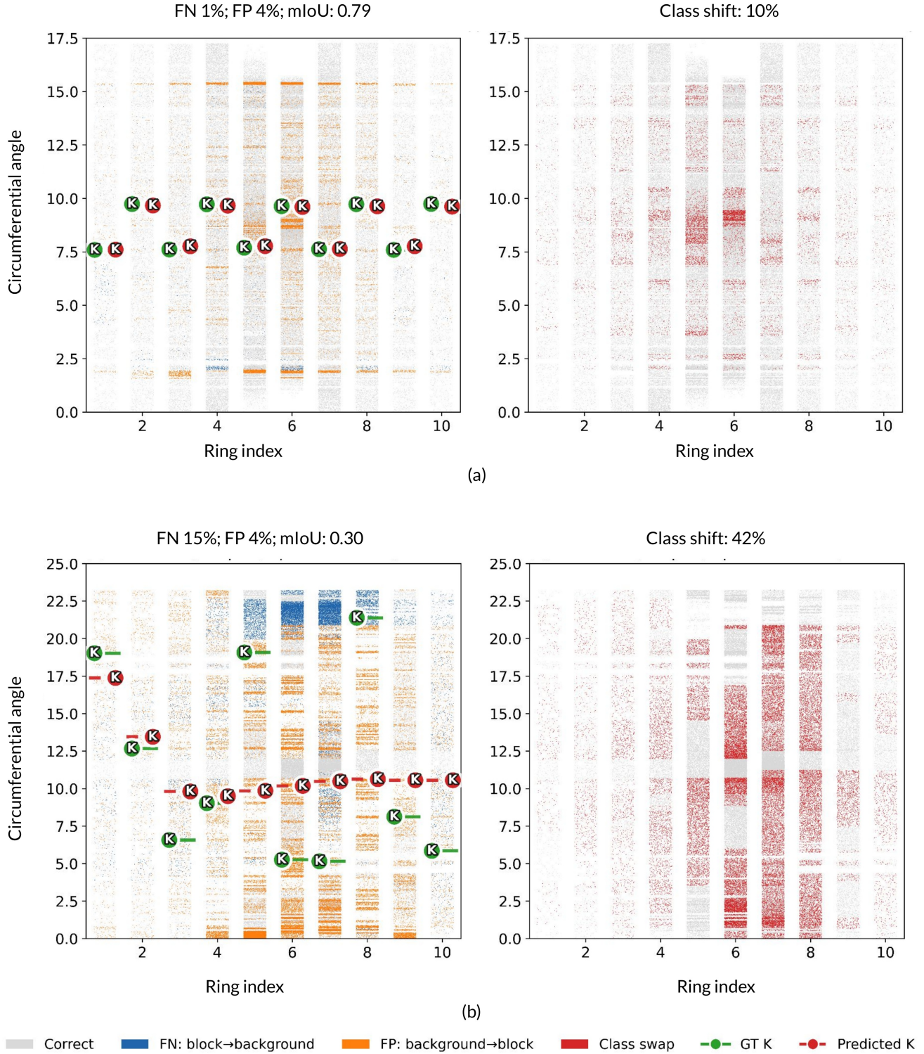
Figure 12: Per-point error maps for a representative regular tunnel (a, regular tunnel 2-1) and complex tunnel (b, complex tunnel 5-1) under m + s + k (Opus-4.6), drawn on the unfolded surface (x: ring index; y: circumferential angle). Left column —detection outcomes: correct (grey), false negatives (blue, segment→background) and false positives (orange, background→segment), with the ground-truth K (green) and predicted K (red) overlaid per ring; titles give FN, FP, and mIoU. Right column —class swaps (red) among otherwise correctly located points. On the regular tunnel the predicted K stays on the GT K and swaps remain low (10%). On the complex tunnel the predicted K is nearly constant and drifts away from the GT K, which jumps ring-to-ring; each affected ring's labels then rotate together and swaps rise to 42%. The maps localise the two constraints: the K mismatch (left) drives the moving-anchor errors, and the resulting label rotation (right) is the dominant residual error.
