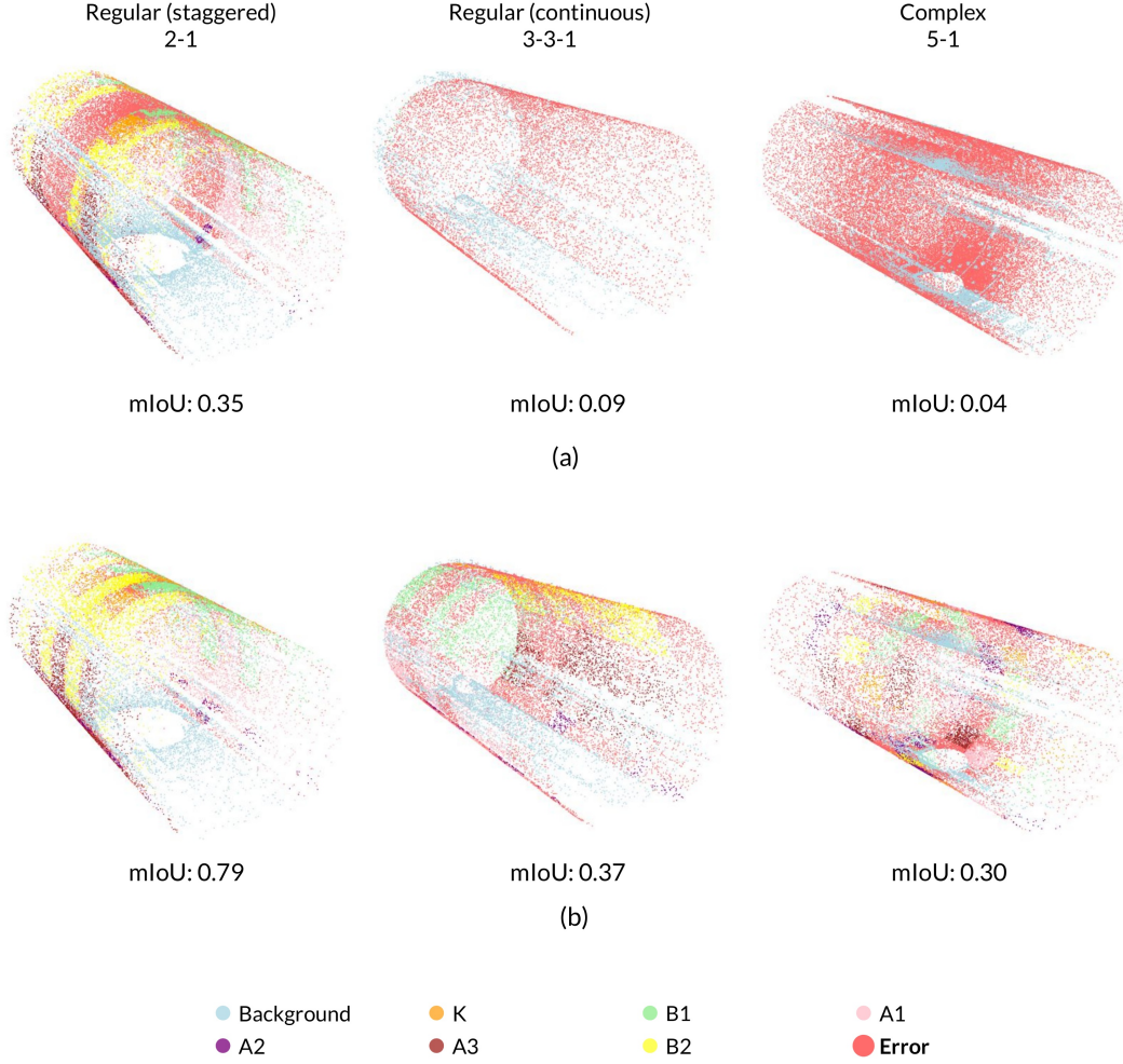
Figure 9: Point-cloud visualisation for the tunnels with the largest mIoU gain in each category: regular (staggered; 2-1), regular (continuous; 3-3-1), and complex (5-1)
