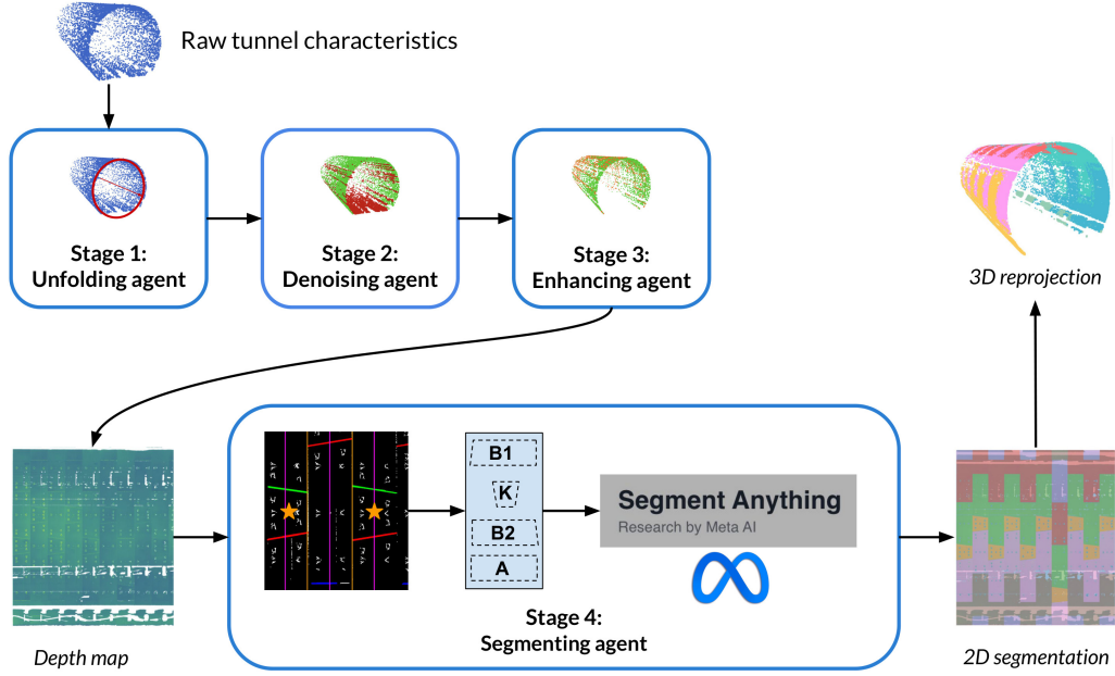
Figure 2: The R4Tun multi-agent architecture for tunnel segmentation. Four blue-boxed stage agents (Stage 1: Unfolding, Stage 2: Denoising, Stage 3: Enhancing, and Stage 4: Segmenting) adapt their stage-specific parameters via LLM reasoning, passing intermediate outputs forward to produce the final segmentation. Arrows indicate the workflow direction from the raw point cloud through intermediate representations to 2D segmentation and 3D reprojection.
