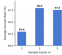
Fig. 4: cIMLE sample factor ablation. LIBERO success averaged across all four suites at H=10 for varying sample factor m . m=1 reduces cIMLE to standard regression (no mode-covering) and drops sharply; m=2 and m=5 are nearly identical, so we use m=2 .
