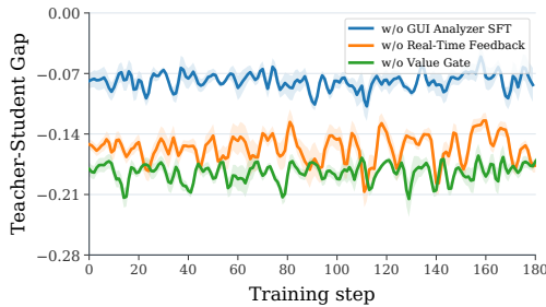
Figure 6: Teacher–student gap throughout training under different ablations of ComputerSD.
