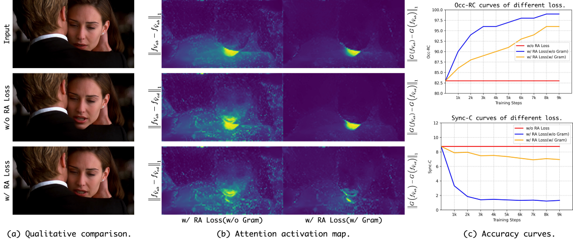
Figure 6. Ablation Study for the Relational Alignment Loss.
