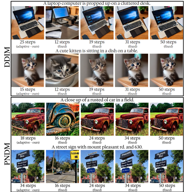
Fig. 5: Text prompts from COCO and images generated by our ADSC, and schedulers fixed number of steps.
