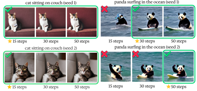
Fig. 1: Effect of text prompt and seed combinations on diffusion steps for generating visually sufficient images. Step counts shown are examples; optimal steps may vary.
