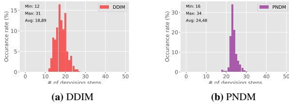
Fig. 4: Distribution of steps upon controlling DDIM and PNDM schedulers using our ADSC in COCO dataset.
