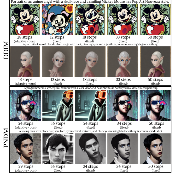
Fig. 7: Text prompts from DiffusionDB and images generated by our ADSC, and schedulers with fixed numbers of steps.
