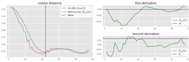
Fig. 3: Plot of cosine distance between total and unconditional noise estimates across diffusion steps, along with first and second derivative curves, for a sample from the DiffusionDB dataset. The X-axis represents the diffusion steps.
