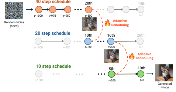
Fig. 2: The denoising process begins with the longest schedule (e.g., 40 steps in the example) and transitions to shorter schedules (20 followed by 10) upon detecting convergence.
