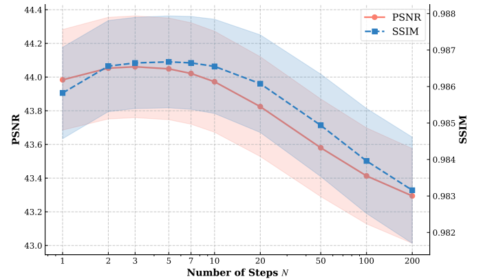
Fig. 7. Impact of step number ( N ) on denoising quality with uniform Schedule. Plots of PSNR (left y-axis, red line) and SSIM (right y-axis, blue dashed line) versus the number of steps ( N ) for the proposed 3D Flow model using a uniform sampling schedule ( k = 0 ) on 1/20 dose of the UDPET dataset. Shaded areas represent standard deviation.
