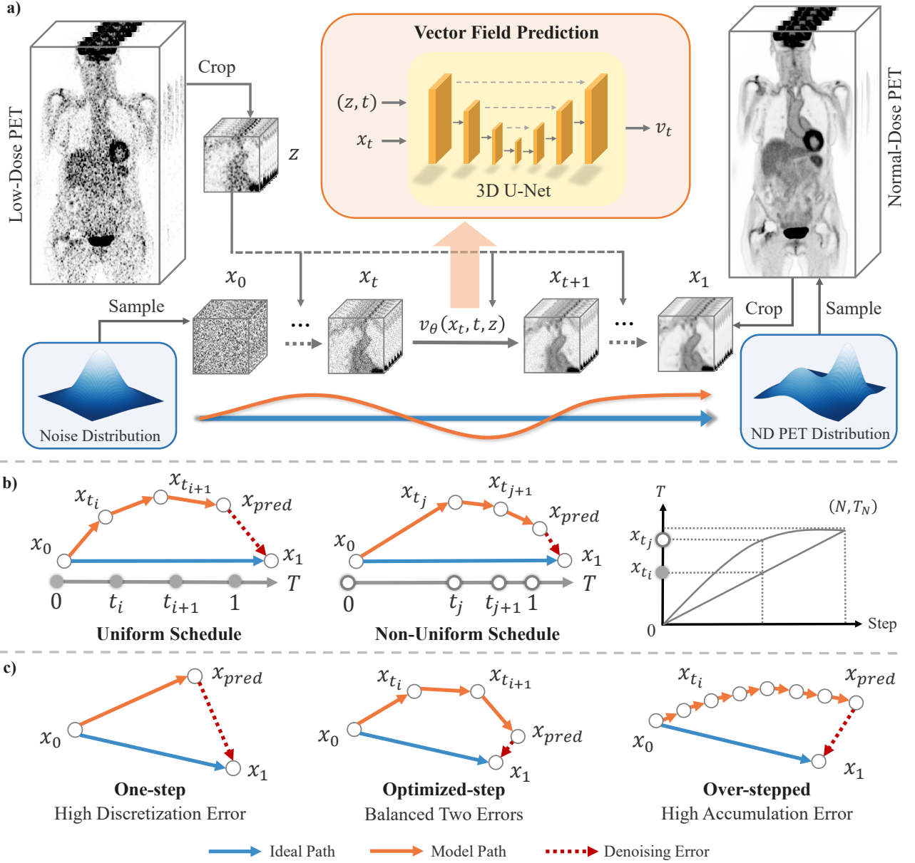
Fig. 1. Overview of the proposed 3D rectified flow denoising framework with an optimized sampling strategy. a) Model Workflow: Our framework utilizes a 3D U-Net to predict a conditional vector field v_\theta(x_t, t, z) , which transports the initial noise ( x_0 ) to the target high-quality PET image ( x_1 ), guided by low-dose input ( z ). Note the deviation between the theoretical straight path (blue arrow) and the actual learned trajectory (orange curve). b) Schedule optimization: The standard uniform sampling schedule (left) is contrasted with the proposed non-uniform schedule (middle). As schematically illustrated by the trajectory curve (right), the non-uniform strategy adjusts the density of time steps along the trajectory and is designed to allocate more integration resolution to selected portions of the path. c) Denoising errors with varying steps: The diagram depicts the distinct error mechanisms observed at varying step counts. A one-step approach (left) suffers from high discretization error due to trajectory curvature. Conversely, an over-stepped approach (right) may accumulate small prediction or integration errors over repeated updates, leading to gradual endpoint drift while generally progressing toward the target. The optimized strategy (center) is designed to balance these two opposing error sources.
