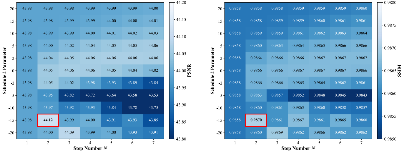
Fig. 8. Heatmaps of PSNR and SSIM for varying step number ( N ) and schedule parameter ( k ). These heatmaps illustrate the combined impact of the total number of steps ( N , x-axis) and the non-uniform sampling parameter ( k , y-axis) on denoising quality (PSNR on left, SSIM on right) for 1/20 dose of the UDPET dataset. Higher values (lighter colors) indicate better performance. The highest performance is highlighted by a red box, achieved at N=2 and k=-15 .
