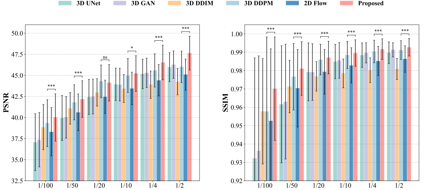
Fig. 4. Quantitative performance on UDPET dataset. Bar plots showing PSNR and SSIM values (mean \pm standard deviation) for different denoising methods across six low-dose levels (1/100 to 1/2) on the UDPET dataset. The proposed 3D rectified flow achieved favorable scores across the evaluated dose levels. Statistical significance (Wilcoxon signed-rank test against the next best baseline) is indicated: * for p < 0.05 , ** for p < 0.01 , and *** for p < 0.001 . ns denotes not significant.
