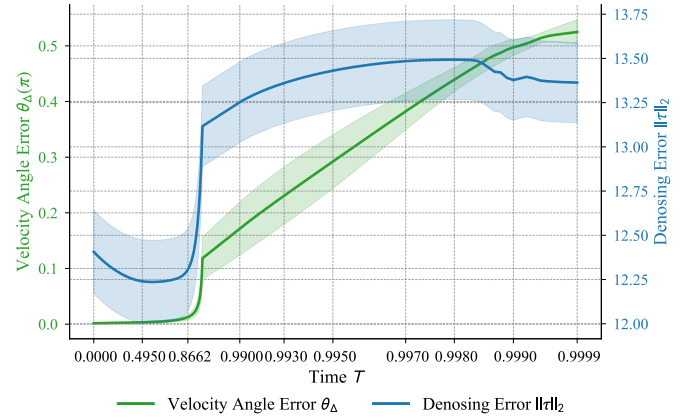
Fig. 10. Plot of velocity angle error ( \theta_\Delta , green, left y-axis) and denoising error ( \|\tau\|_2 , blue, right y-axis) over time ( T , x-axis) for a 3D Flow trajectory. Shaded areas indicate standard deviation. For the denoising error ( \tau , blue), the shaded area is scaled by a factor of 0.05 for visualization purposes.
