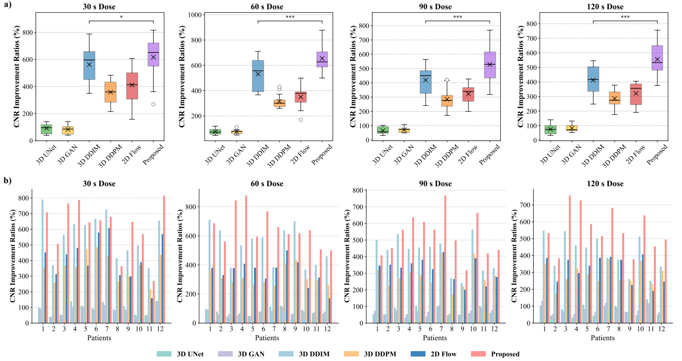
Fig. 6. Local lesion CNR improvement on FAHZU dataset. a) Overall CNR improvement ratios: Box plots illustrating the distribution of CNR improvement ratios for various denoising methods across four dose levels (30 s, 60 s, 90 s, 120 s) on the FAHZU dataset. CNR is influenced by both lesion-background contrast and background variance and should be interpreted together with global image-quality metrics and visual assessment. Statistical significance (Wilcoxon signed-rank test against the next best baseline) is indicated: * for p < 0.05 , ** for p < 0.01 , and *** for p < 0.001 . b) Patient-specific CNR improvement ratios: Bar plots showing the CNR improvement ratios for 12 individual patients across different dose levels (30 s, 60 s, 90 s, 120 s) and various denoising methods.
