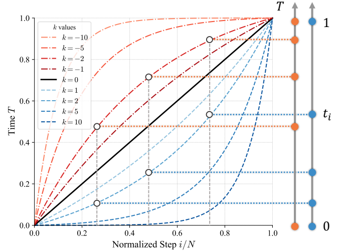
Fig. 2. Illustration of non-uniform sampling schedules controlled by the hyperparameter k . This figure shows the distribution of time steps t_i as a function of the normalized step index i/N for various values of the hyperparameter k .
