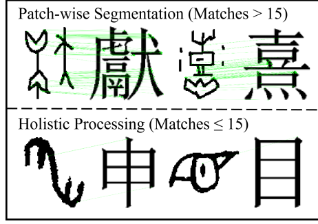
Fig. 1. Training-time gating mechanism for OBS (left) and modern characters (right). Top: dense keypoint matches ( n_{\text{match}} > \gamma ) trigger patch-wise local segmentation for radical alignment. Bottom: sparse matches ( n_{\text{match}} \leq \gamma ) lead to holistic processing to preserve global character topology, where \gamma = 15 .
