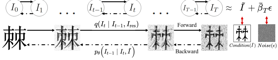
Fig. 2. Steps of the residual denoising diffusion model.
