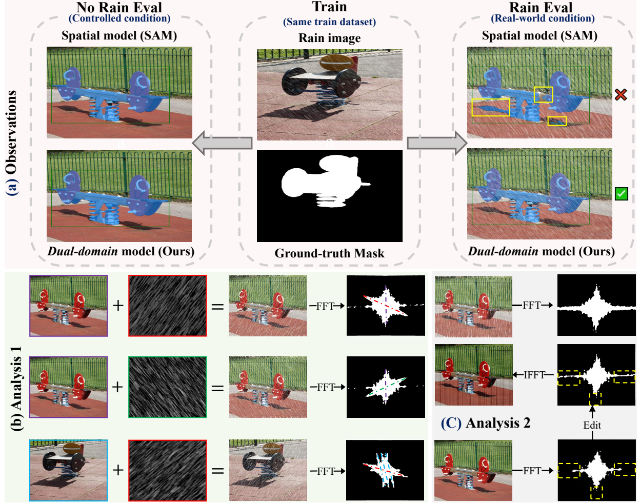
Fig. 2. Motivation for Frequency-Aware Modeling. (a) Robustness Comparison: Contrast between spatial-only models (SAM) and our dual-domain approach under controlled vs. real-world noisy conditions. (b) Spectral Analysis: Illustration of distinct directional energy distributions for global noise patterns, highlighting their consistency across varying objects. (c) Global Governance: Visualization of global spatial structural distortions induced by local frequency component editing.
