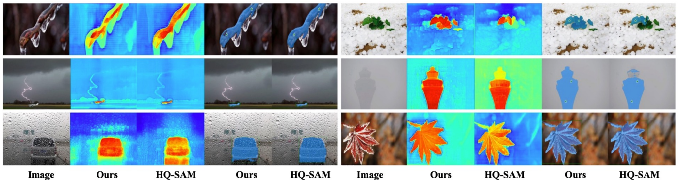
Fig. 8. Visual comparison of cross-attention heatmaps between the original HQ-SAM output token and the FSANet output token in the final decoder layer. FSANet demonstrates stronger focus on object boundaries and structural regions that are misclassified by the original token.
