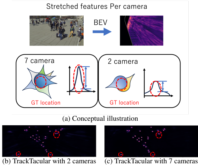
Fig. 3. Effect of camera count on BEV projection. Directional spreading is more visible with two cameras, while additional views produce more concentrated BEV responses.
