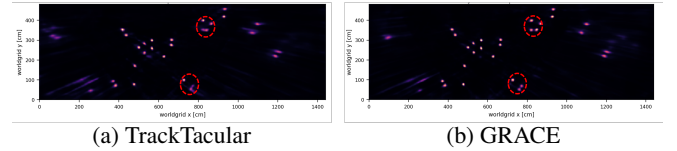
Fig. 7. BEV responses with the same two WildTrack cameras. TrackTacular shows directional spreading around several pedestrians, while GRACE produces more concentrated responses. Red circles highlight representative differences.
