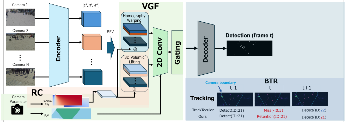
Fig. 2. GRACE overview. VGF fuses projected and lifted features using coverage and ray geometry. BTR lets low-confidence detections continue existing tracks through short score drops.
