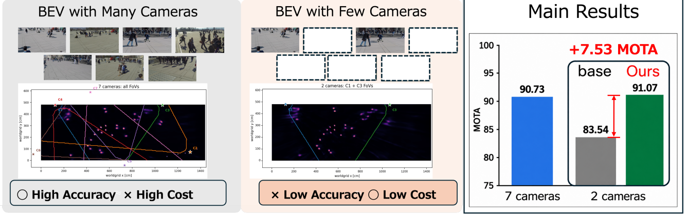
Fig. 1. Few-camera tracking on WildTrack. GRACE reaches 91.07 MOTA with only two cameras, compared with 83.54 for two-camera TrackTacular. The 90.73 seven-camera bar uses VGF + Ray detections with the default tracker.
