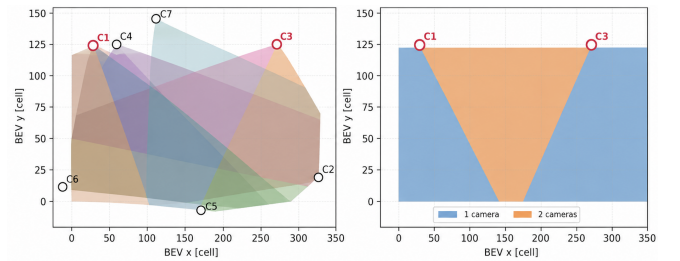
Fig. 5. WildTrack camera configuration. The left panel shows the positions and fields of view of all seven cameras. The right panel shows the selected C1+C3 pair. Blue regions are observed by one camera and the orange region by both cameras. C1+C3 covers the complete BEV evaluation area, with 44.98% observed by both cameras.
