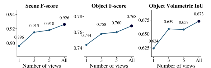
Fig. 8. Study on Multi-view Condition on the Scan2CAD Dataset.
