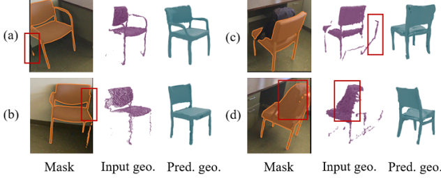
Fig. 7. Qualitative Results under Perception Noise.
