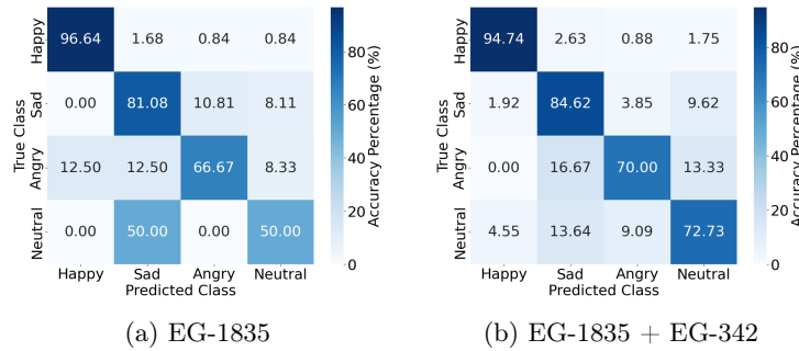
Fig. 4: Comparison of Confusion Matrices for Models Trained on Different Datasets
