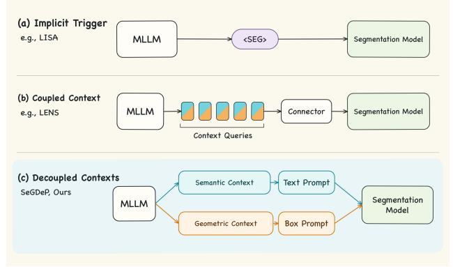
Figure 1: Reasoning-to-segmentation interfaces. Trigger and coupled-context designs provide no explicit separation; SeGDeP emits complementary semantic and box prompts.
