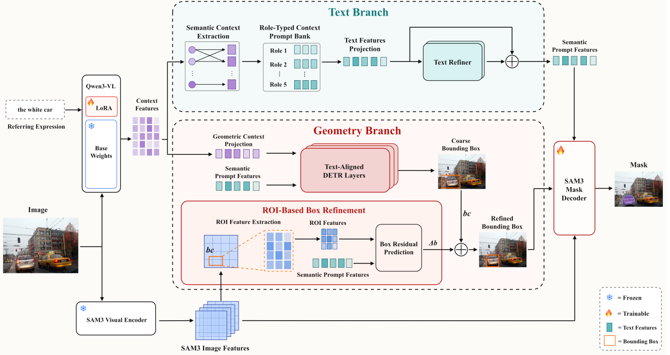
Figure 2: Architecture of the Qwen3-VL/SAM 3 instantiation of SeGDeP. A role-typed semantic branch produces P_{\text{sem}} , while an independent projection produces geometric context Z_{\text{geo}} . Both condition DETR to predict b_c , which selects frozen SAM 3 ROI features for residual refinement. The decoder combines semantic features, the refined box, and image features. Snowflakes and flames denote frozen base weights and trainable adapters or decoder components, respectively; all newly introduced modules are trainable.
