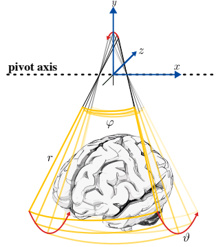
Figure 5: Geometry of the 3D acquisition. A mechanically swept probe is modelled as a curvilinear 2D array (yellow fan) rotated about an internal pivot axis (dashed), so that a voxel is addressed by depth r and two angular coordinates: \varphi within the fan and \vartheta about the pivot. Each scanline is treated as an independent propagation path.
