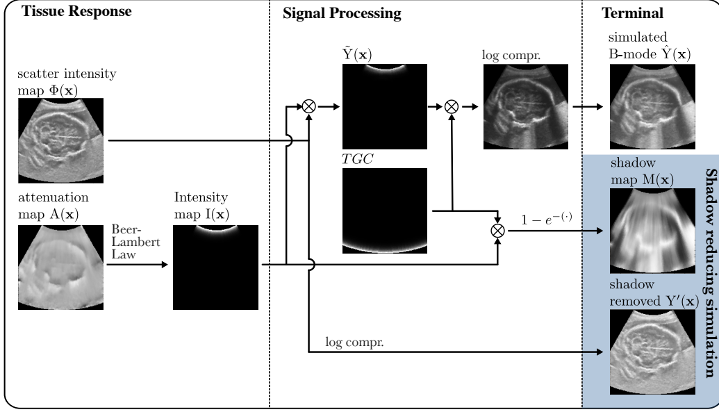
Figure 6: Visual representation of the differentiable simulation pipeline as defined by eq. (1)–eq. (10). The first target (top right) is the simulated ultrasound image \hat{Y} , while the lower two targets are the shadow-reduced image Y' and the shadow map M , which are only relevant after the tissue parameters have been estimated (b in Figure 3).
