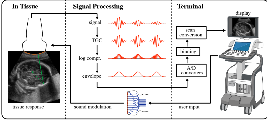
Figure 4: The canonical ultrasound imaging pipeline on which RFlash is built. Tissue response (left) is modulated by the propagating sound field, then processed in the scanner (centre: envelope detection, time-gain compensation, log compression) and converted to a display image (right: A/D conversion, binning, scan conversion). RFlash operates on the displayed, beamformed image and inverts the shaded operations. A/D conversion and binning are lossy and are not modelled. Compare with Figure 6, which shows the corresponding differentiable pipeline for beamformed images.
