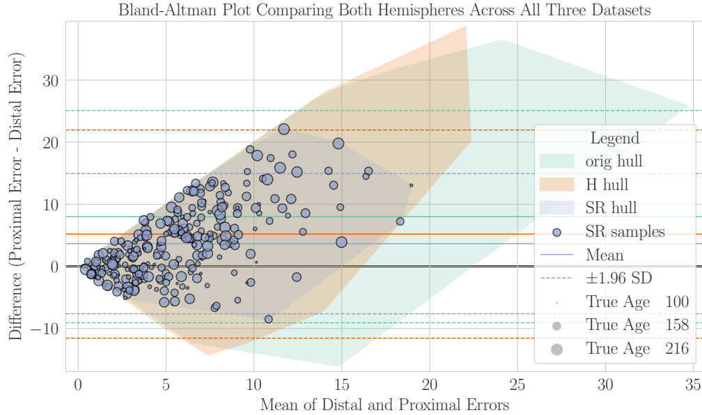
Figure 8: Bland–Altman plots for age prediction on both hemispheres across the three datasets: the original images (orig), the images with Hughes shadow reduction (H), and the images with RFlash shadow reduction (SR). For readability, the first two datasets show only the convex hull, mean, and standard deviation. The full results are provided in Section Appendix A.2.
