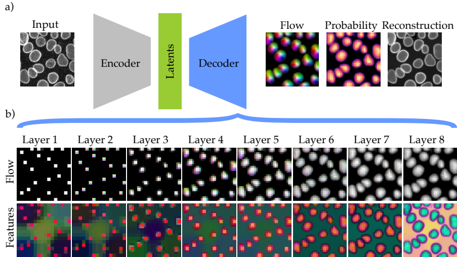
Fig. 1: Overview of Generative Routing Pyramids. a) From an input image, the encoder predicts a latent field, which is then used to generate pyramidal (coarse-to-fine) flows to reconstruct the image. b) Per-layer flow and routed feature maps. The flows are shown as HSV encoding, where hue is the flow direction, saturation is the flow magnitude, and value is the routed probability mass. The features are shown as RGB values representing the first three principle components.
