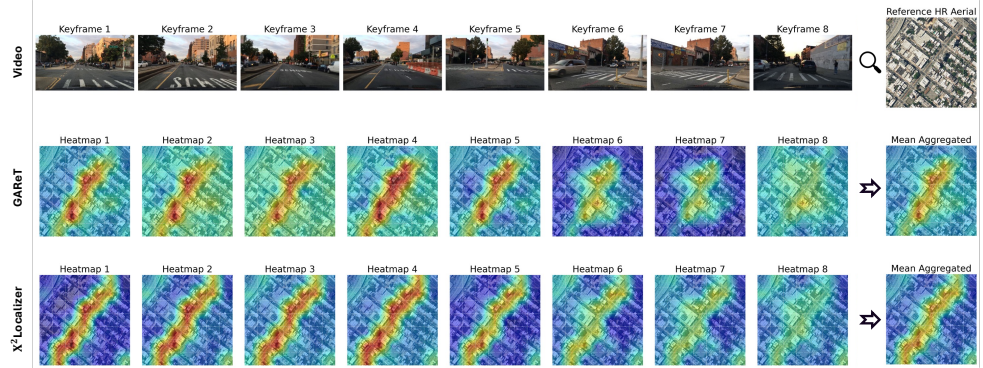
Figure 5: Qualitative visualization of frame-level localization cues. We show representative key frames, the corresponding aerial reference image, and the heatmaps produced by GARET and X^2 Localizer. X^2 Localizer yields sharper and more temporally consistent responses across key frames, suggesting that asymmetric cross-grained alignment helps aggregate reliable local evidence for progressive localization.
