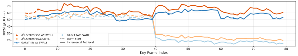
Figure 4: Long-range localization on the challenging subset. We compare our proposed method against GARET, both with and without SWRL, which supports short warm-start and periodic re-localization via SWRL. Dashed lines indicate warm-up and backward refinement performance, whereas solid lines denote incremental frame-level refinement after activation.
