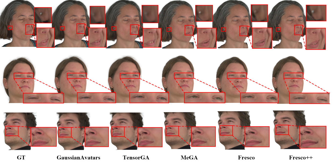
Fig. 2. Qualitative comparison on self-reenactment. Fresco++ better preserves subject-specific appearance details and reproduces expression-dependent local structures, such as earrings, eye opening, and cheek wrinkles, under unseen facial motions.
