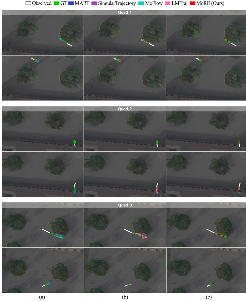
Figure 12: Visualization of prediction results on the quad_1, 2, 3 scenes. To aid visualization, selected agents are shown.
