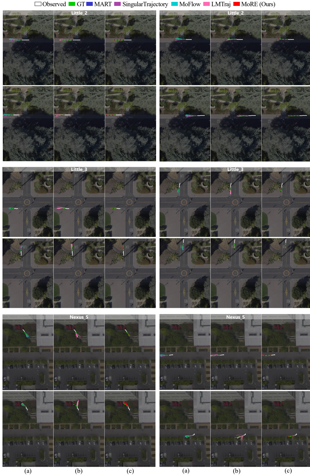
Figure 14: Visualization of prediction results on the little_2, 3 and nexus_5 scenes. To aid visualization, selected agents are shown.
