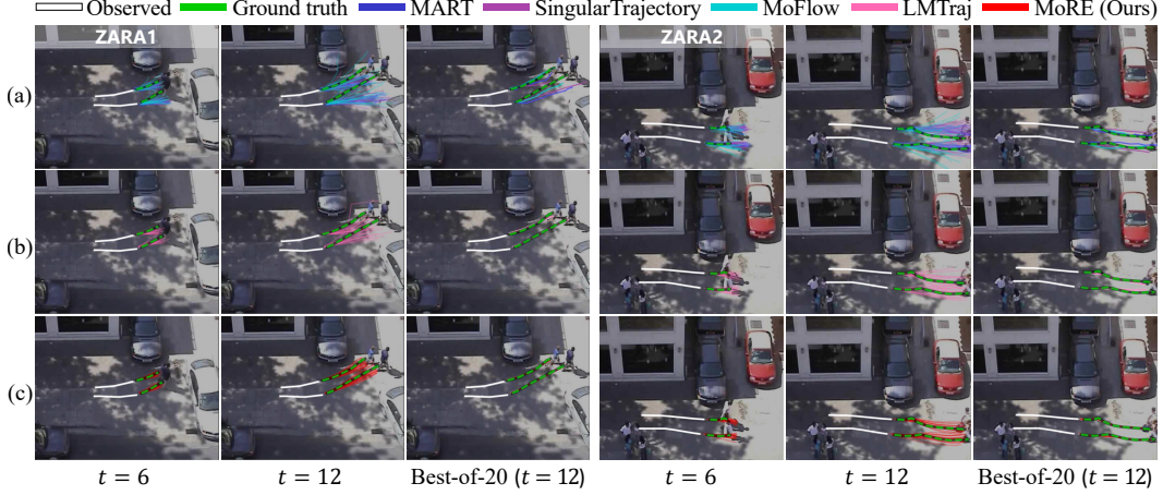
Figure 3: Sampled predictions on ZARA1 and ZARA2 at t = 6 and t = 12 , with the best-of-20 trajectory. Rows show (a) numerical baselines, (b) LMTraj, and (c) MoRE. Additional qualitative results are provided in Sec. E.
