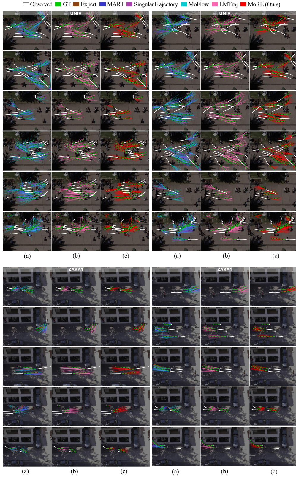
Figure 6: Visualization of prediction results on the UNIV and ZARA1 scenes. To aid visualization, selected agents are shown.
