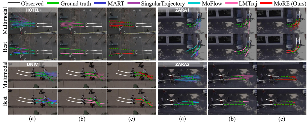
Figure 1: Prediction examples on ETH-UCY. “Multimodal” shows 20 samples, and “Best” shows the closest sample. (a) Numerical baselines and (b) LMTraj exhibit different spatial patterns. (c) MoRE refines the language-based predictions using numerical feedback.
