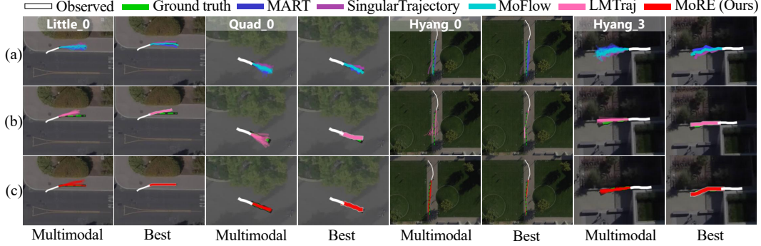
Figure 4: Sampled predictions on four SDD scenes, showing 20 trajectories and the best-of-20 trajectory. From top to bottom, rows show numerical baselines, LMTraj, and MoRE.
