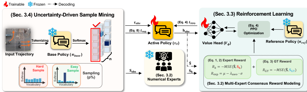
Figure 2: MoRE training pipeline. A frozen base policy ranks training samples by predictive entropy. Numerical expert predictions for the selected subset are cached once. Decoded policy samples receive expert-consensus and ground-truth rewards for PPO refinement, interleaved with supervised learning. Only the refined forecasting policy is needed at inference.
