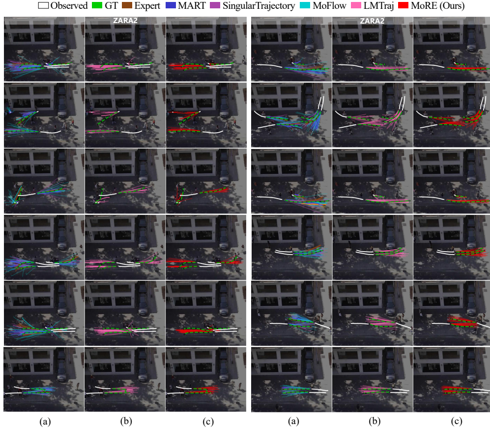
Figure 7: Visualization of prediction results on the ZARA2 scene. To aid visualization, selected agents are shown.
