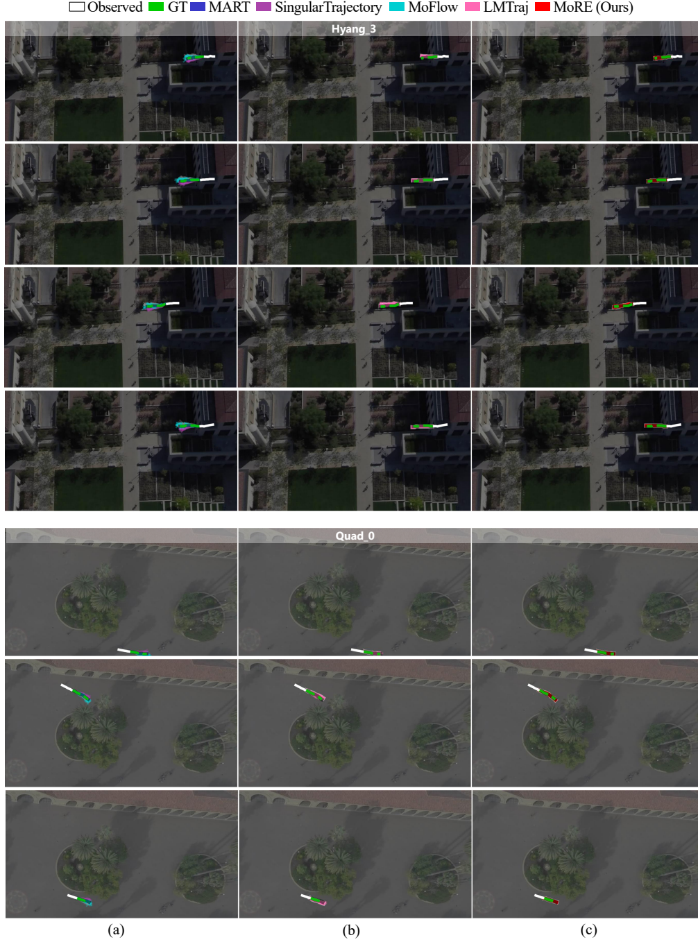
Figure 11: Visualization of trajectory predictions on hyang_3 and quad_0 scenes. To aid visualization, selected agents are shown.
