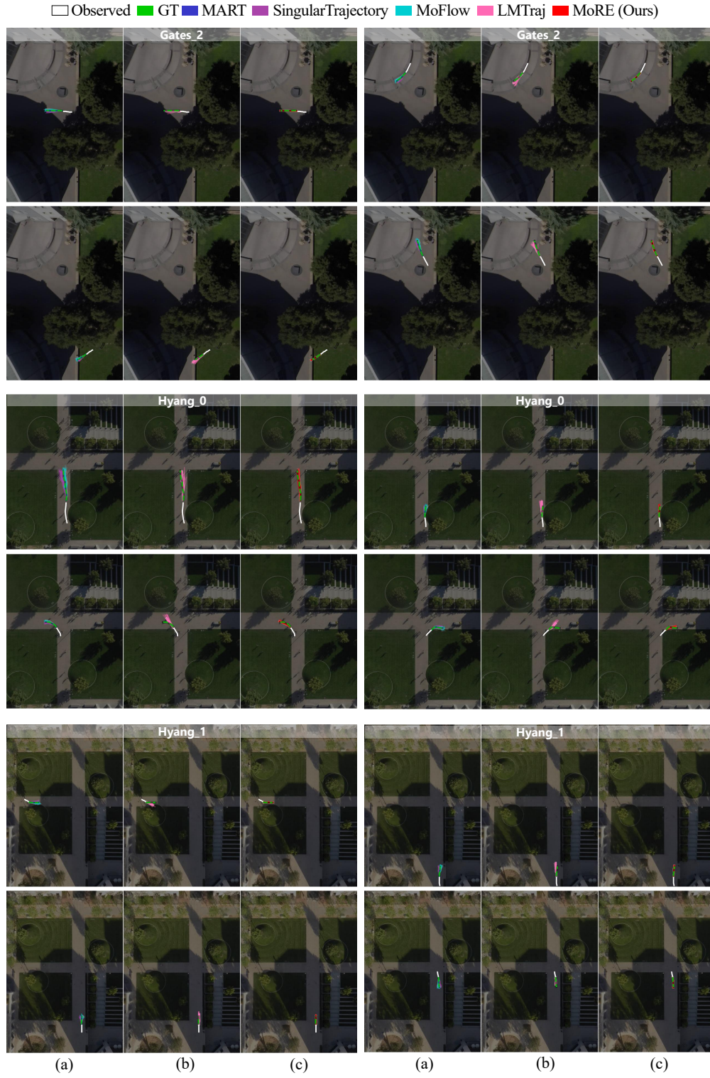
Figure 9: Visualization of trajectory predictions on gates_2, hyang_0, 1 scenes. To aid visualization, selected agents are shown.
