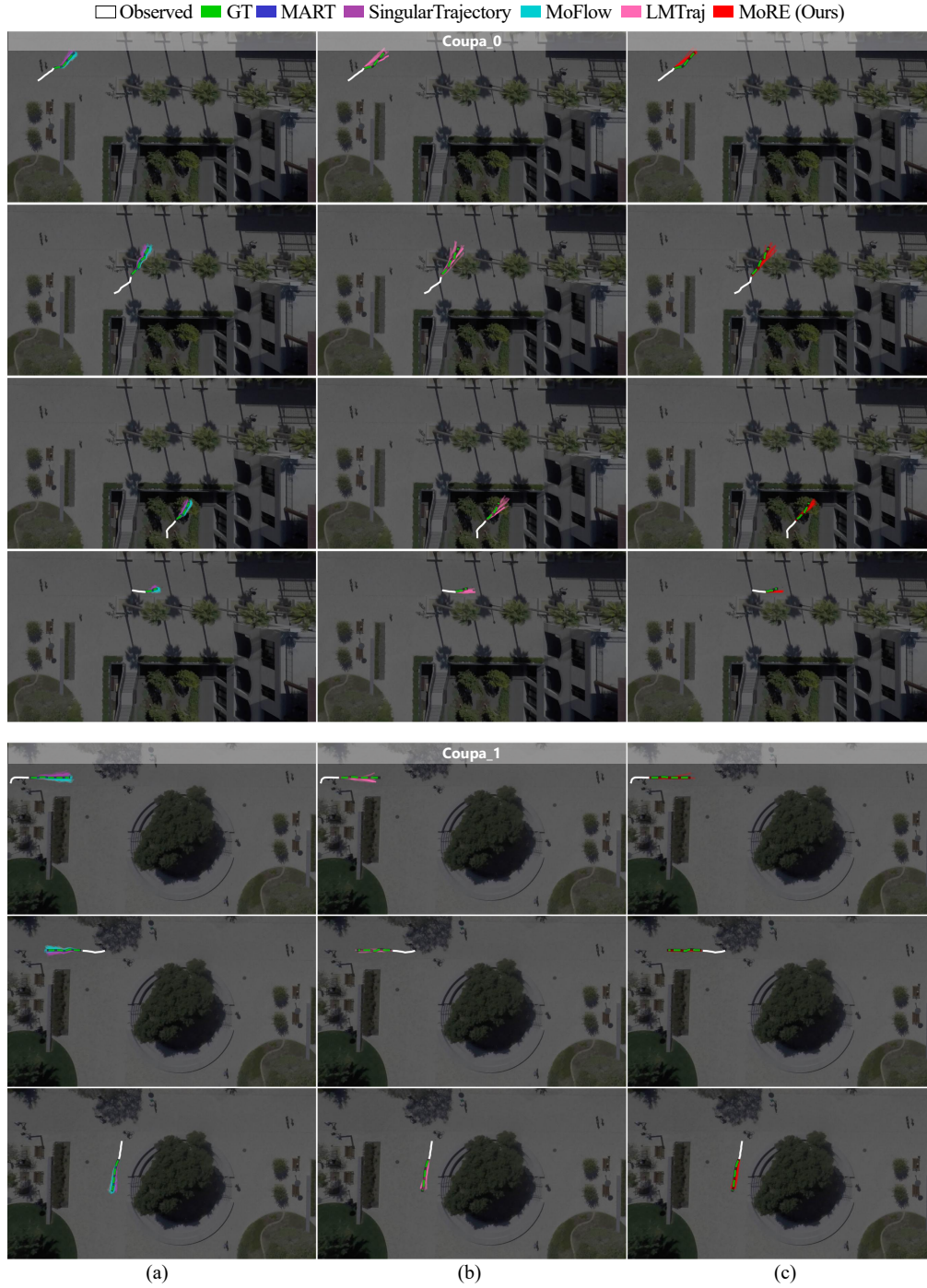
Figure 10: Visualization of prediction results on the coupa_0 and coupa_1 scenes. To aid visualization, selected agents are shown.
