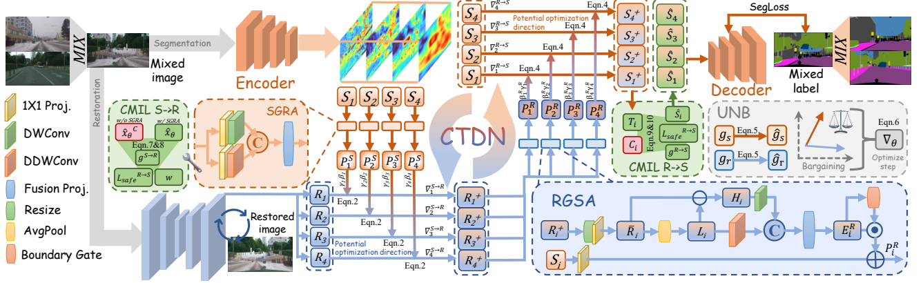
Figure 2. Overview of the proposed Unsupervised Restoration-Segmentation Collaborative Learning Framework (Ultra). Given mixed images from cross-domain sampling, Ultra jointly optimizes image restoration and semantic segmentation through bidirectional cross-task guidance. Specifically, segmentation features S_i are transformed into semantic priors P_i^S by the SGRA, which performs conditional modulation on restoration features to provide potential restoration optimization directions. The modulated restoration features R_i^+ are further converted into restoration priors P_i^R through the RGSA, providing potential segmentation optimization directions via conditional modulation. UNB selects the optimal cross-task optimization directions during training. To mitigate the Self-reinforcing Hallucination Loop in unsupervised cross-task collaboration, CMIL estimates the causal effects of semantic and restoration interventions and only propagates beneficial interventions.
