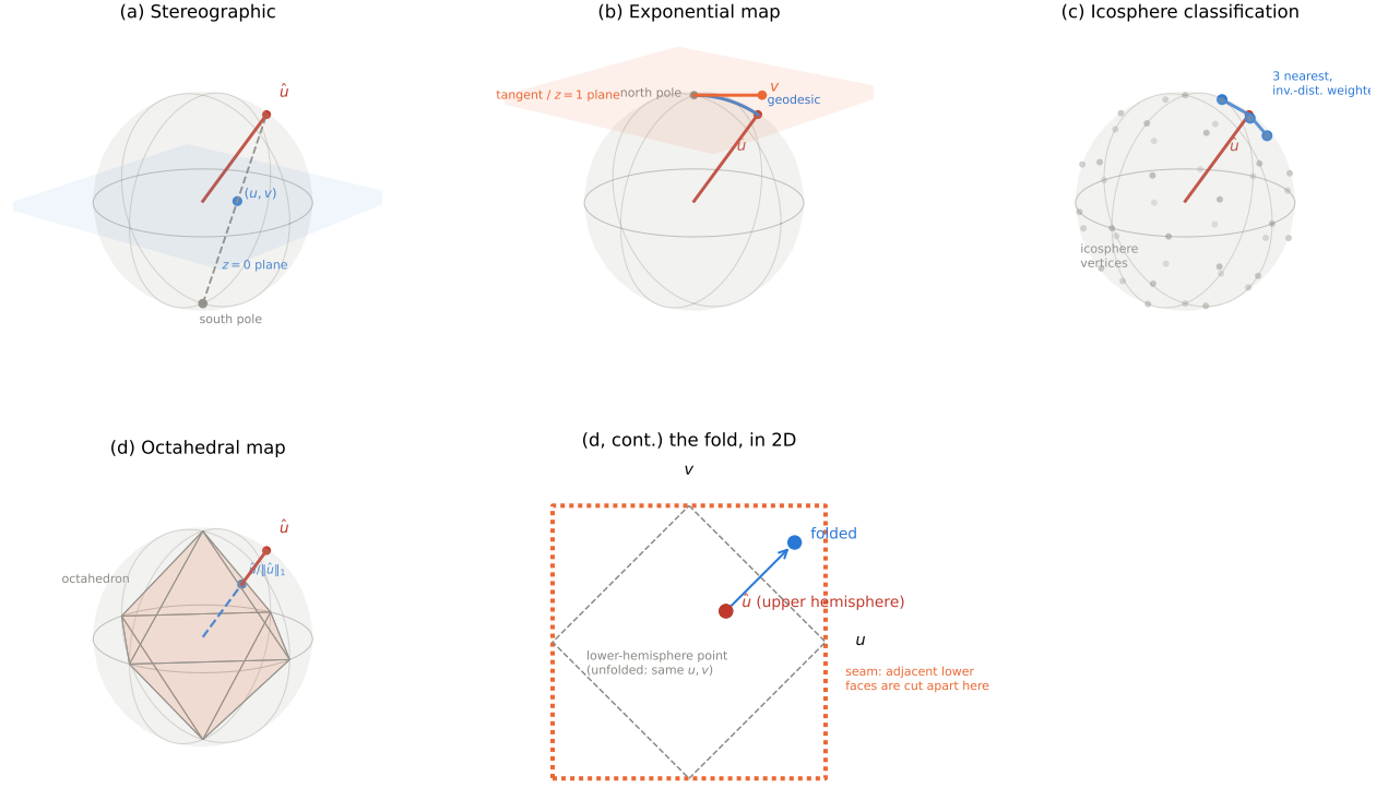
Figure 1: The four representations that are hardest to picture from the description above, all shown for the same example up-axis \hat{u} (red). (a) Stereographic: projection from the south pole onto the plane z = 0 . (b) Exponential map: the tangent-plane vector v at the north pole and its corresponding geodesic (blue) on the sphere. (c) Icosphere classification: the discretized vertex set, with the three nearest vertices (blue) weighted by inverse distance. (d) Octahedral map: radial projection onto the unit- L_1 octahedron (left), and why the fold is needed (right): without it, \hat{u} and the marked point on the opposite (lower) hemisphere would land on the identical (u, v) . Folding the lower hemisphere into the square’s free corners removes the ambiguity.
