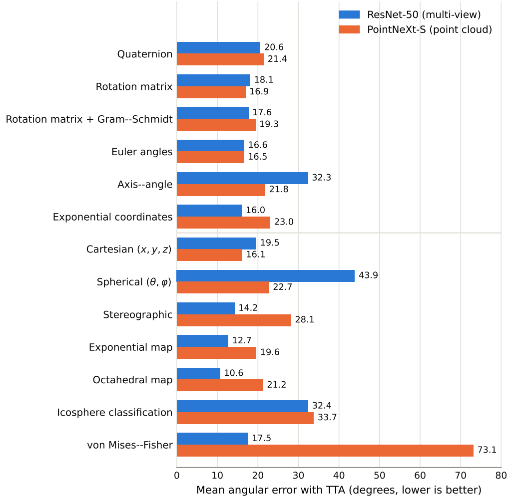
Figure 2: Mean angular error with TTA (test set, K = 21 icosphere rotations), by representation and backbone. Lower is better. The top six representations parameterize the full rotation ( SO(3) ); the bottom seven target the up-axis directly ( S^2 ).
