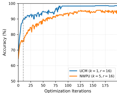
Fig. 4: Accuracy (%) evolution of SE-CLIP across 200 iterations on the UCM and NWPU benchmarks. The grey dashed vertical line marks the mining onset.
