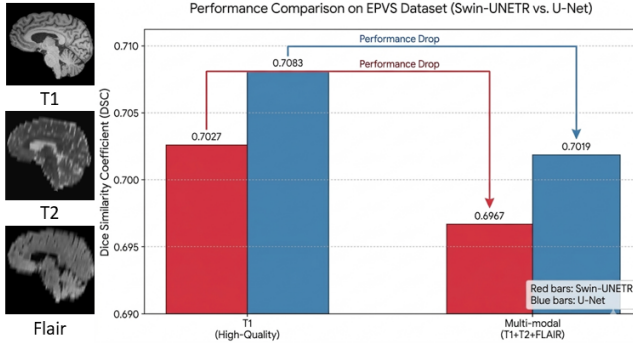
Figure 1: Illustration of multi-modal fusion performance. Left: Visual comparison of high-resolution T1, low-resolution T2, and FLAIR modalities. Right: Quantitative results showing a performance drop in standard architectures when transitioning from T1-only inputs to multi-modal inputs.
