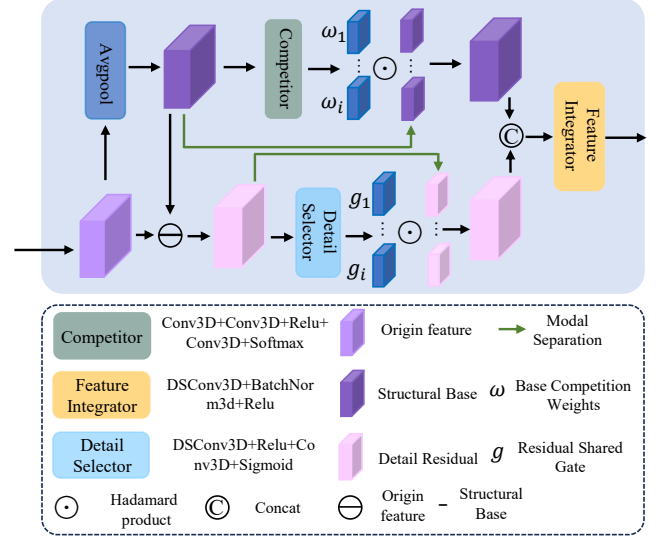
Figure 5: Inter-Modal Spatial-Scale Harmonization. The IMSH module explicitly decouples multi-modal inputs into macroscopic structural bases and detail-sensitive residuals via spatial filtering, suppressing physical noise before deep semantic interaction.
