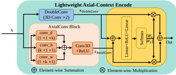
Figure 4: Lightweight Axial-Context Encoder. Features from DoubleConv and AxialConv branches are integrated via Selective Fusion, where \oplus and \otimes denote element-wise summation and multiplication for generating and applying adaptive attention weights.
