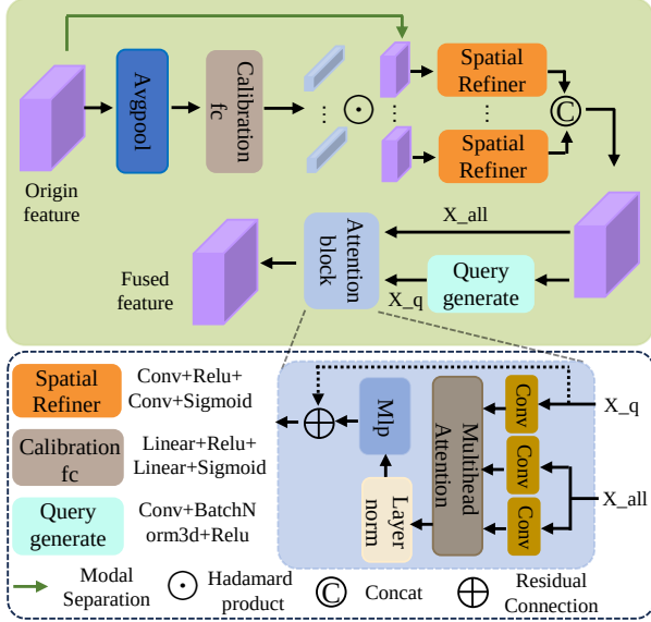
Figure 6: Modality Bias Calibration Fusion. The MBCF module performs hierarchical channel and spatial calibration to resolve deep semantic conflicts between modalities.
