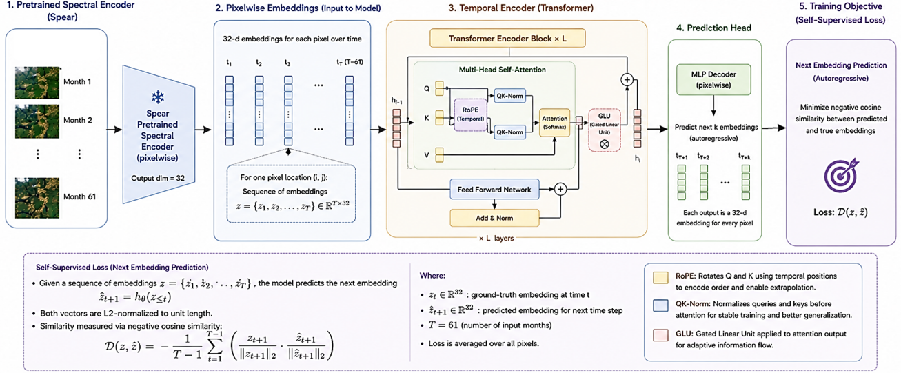
Figure 1. Overview of the proposed SPEAR-NeXT framework. A frozen pretrained SPEAR spectral encoder transforms each multi-spectral pixel observation into a compact 32-dimensional instantaneous spectral state. The resulting pixel-wise embedding sequence is processed by a causal temporal Transformer equipped with Rotary Position Embeddings, QK normalization, and gated feed-forward transformations. Horizon-specific prediction heads directly forecast multiple future latent states, which are optimized using self-supervised horizon-weighted latent trajectory supervision.
