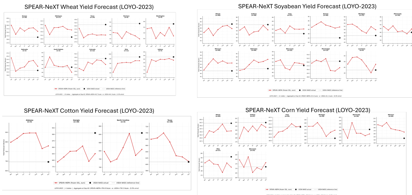
Figure 5. State-wise in-season crop-yield forecasting under the leave-one-year-out 2023 evaluation. Results are shown for (a) wheat, (b) soybean, (c) cotton, and (d) corn. Red trajectories denote SPEAR-NeXT yield predictions generated at successive in-season forecast dates, black markers indicate the final USDA NASS reported yields, and horizontal dashed lines provide the USDA NASS reference level for each state. The value n shown in each panel denotes the number of spatial samples used for the corresponding state. The figure illustrates both the progressive updating of yield estimates during the growing season and the variation in forecasting difficulty across crops and geographic regions.
