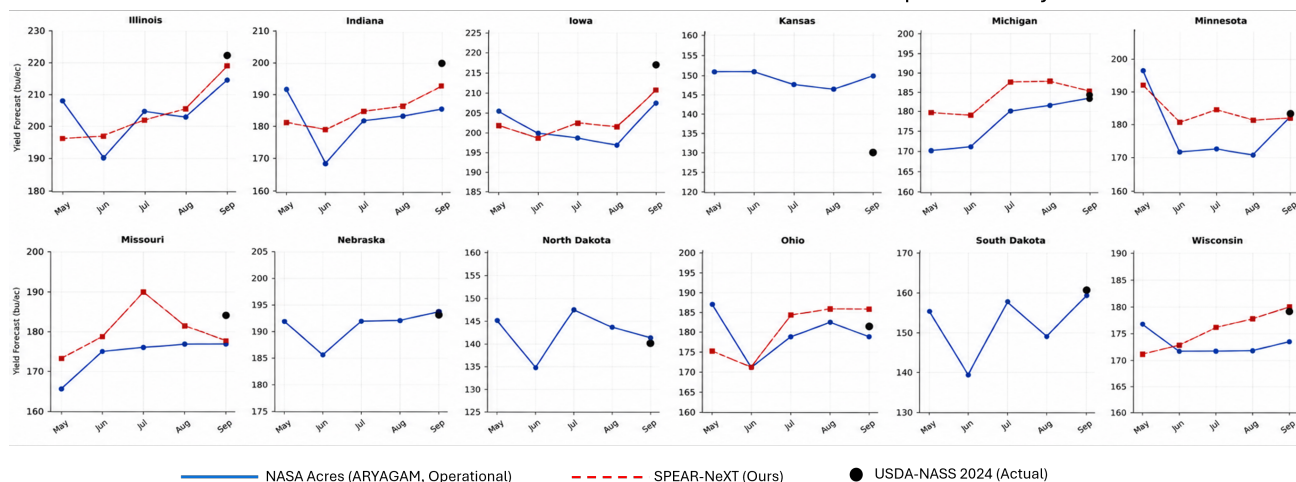
Figure 6. Comparison of 2024 corn-yield forecasts from SPEAR-NeXT and the NASA Acres operational forecasting system across 12 Midwestern states. Blue curves represent the publicly reported NASA Acres forecasts, red curves represent SPEAR-NeXT predictions, and black markers denote the final USDA NASS yield estimates. SPEAR-NeXT produces forecasts using the frozen self-supervised representation and a lightweight downstream yield-prediction head. This comparison is provided as an operational reference rather than a controlled benchmark because the two systems may differ in input data, spatial aggregation, forecast issue dates, preprocessing, and evaluation protocols.
