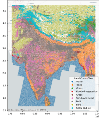
(a) India pretraining corpus for SPEAR, containing approximately 2.7 million pixel-level samples from Sentinel-2, PlanetScope, Sentinel-1, and matched climate–environmental variables.
