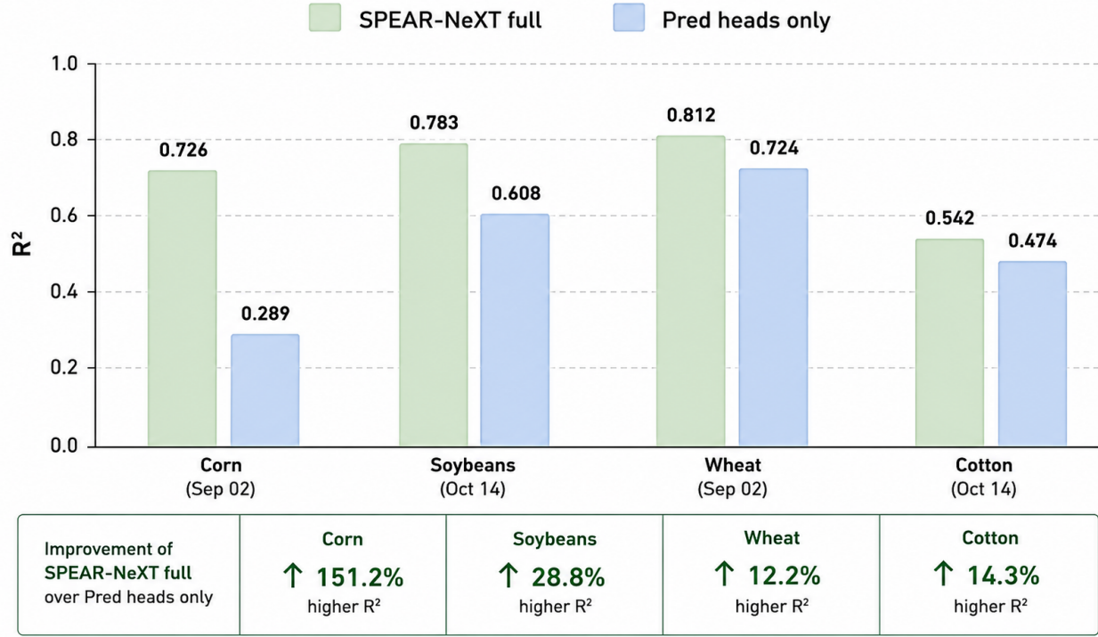
Figure 3. Contribution of the pretrained SPEAR-NeXT temporal representation to crop-yield prediction. Crop-specific R^2 values are compared between the complete SPEAR-NeXT pipeline and a prediction-head-only control at the indicated forecast dates. The complete model combines frozen SPEAR pixel states, the self-supervised SPEAR-NeXT temporal encoder, and the downstream prediction head, whereas the control excludes the pretrained temporal representation and uses only the prediction head. SPEAR-NeXT improves R^2 from 0.289 to 0.726 for corn, from 0.608 to 0.783 for soybean, from 0.724 to 0.812 for wheat, and from 0.474 to 0.542 for cotton. These correspond to relative improvements of 151.2%, 28.8%, 12.2%, and 14.3%, respectively.
