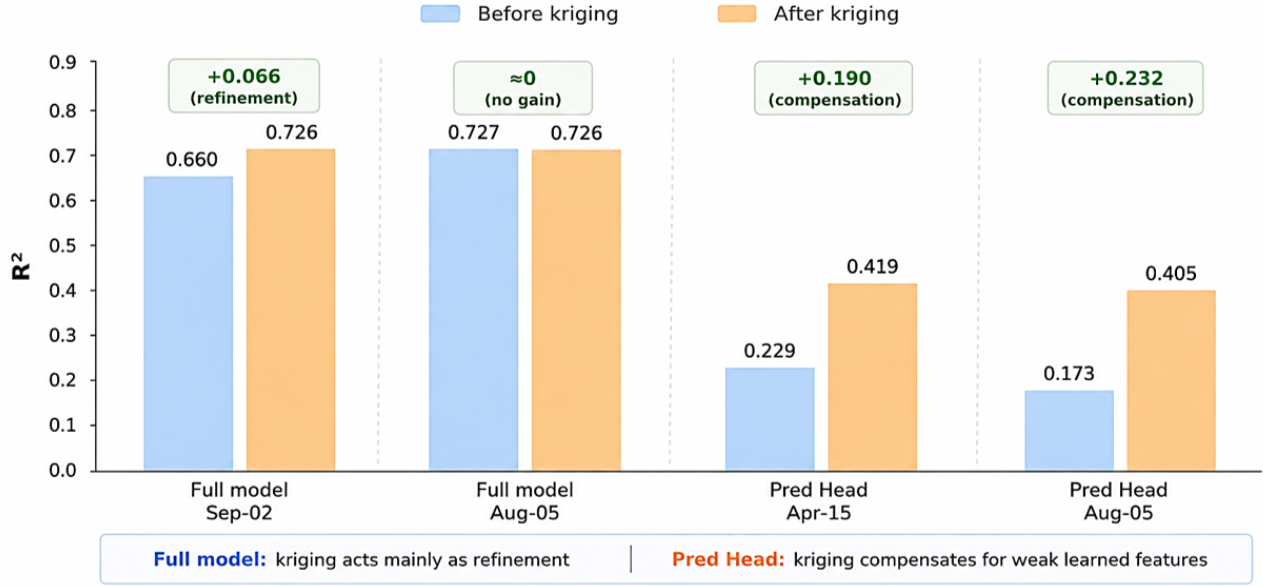
Figure 4. Effect of post-hoc spatial kriging on corn-yield prediction using the complete SPEAR-NeXT model and the prediction-head-only control. The complete model combines the frozen SPEAR encoder, the pretrained SPEAR-NeXT temporal encoder, and the downstream yield-prediction head. The prediction-head-only control excludes the pretrained temporal encoder and uses the same downstream head. Blue bars report performance before kriging, while orange bars report performance after spatial kriging. For the full model, kriging increases R^2 from 0.660 to 0.726 for the September 2 forecast and produces essentially no change for the August 5 forecast (0.727 to 0.726). In contrast, the prediction-head-only configuration improves from 0.229 to 0.419 for the April 15 forecast and from 0.173 to 0.405 for the August 5 forecast. These results indicate that kriging primarily refines the already informative SPEAR-NeXT predictions, whereas it compensates more strongly for the weaker spatial structure learned by the prediction-head-only model.
