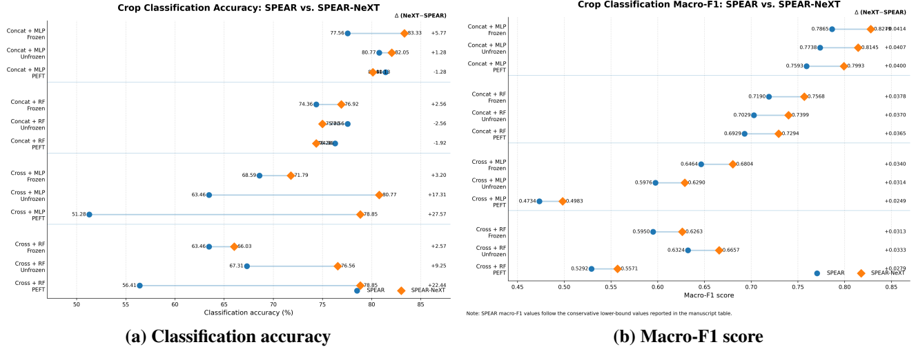
Figure 2. Crop-classification performance of SPEAR and SPEAR-NeXT under different multimodal fusion, prediction-head, and adaptation settings. Each horizontal pair compares SPEAR with SPEAR-NeXT for the same configuration, while the rightmost value reports the corresponding SPEAR-NeXT minus SPEAR difference. Concat denotes feature concatenation, Cross denotes cross-attention-based fusion, MLP denotes multilayer perceptron, RF denotes random forest, and PEFT denotes parameter-efficient fine-tuning. The SPEAR macro-F1 values correspond to the conservative lower-bound values reported in Table 6.
