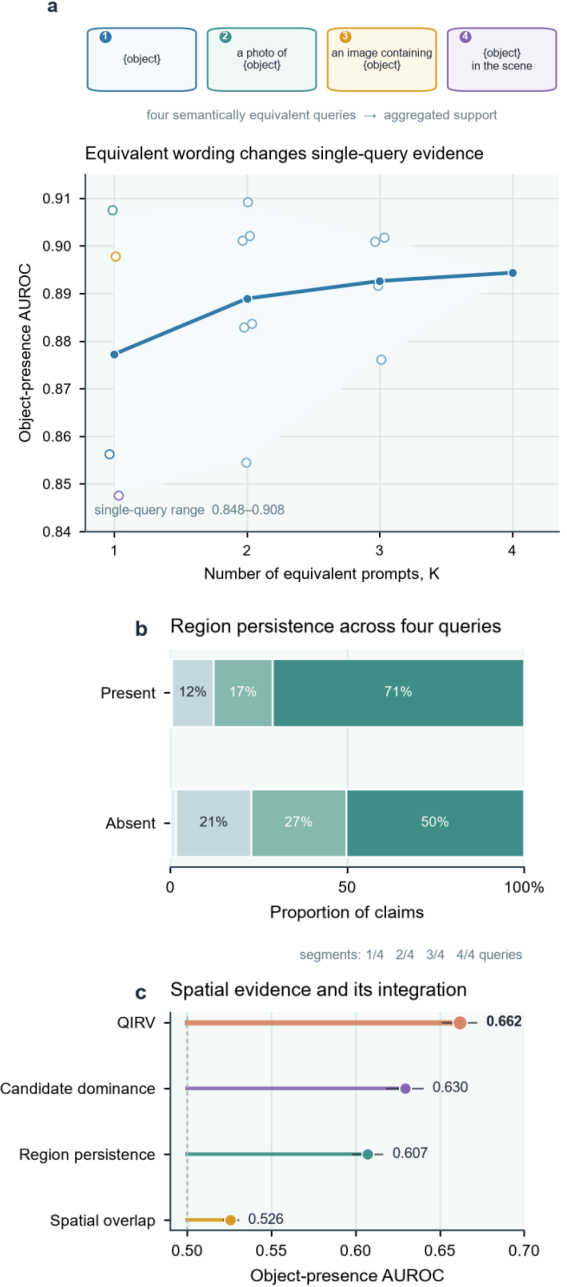
Fig. 2. Empirical motivation for semantic-spatial verification in SSAV. (a) Object-presence AUROC across different numbers of semantically equivalent queries; the line and shaded region show the mean and range across prompt combinations. (b) Distribution of the largest region-cluster size for present- and absent-object claims. (c) Object-presence AUROC of QIRV and its three spatial components, with image-clustered 95% bootstrap confidence intervals.
