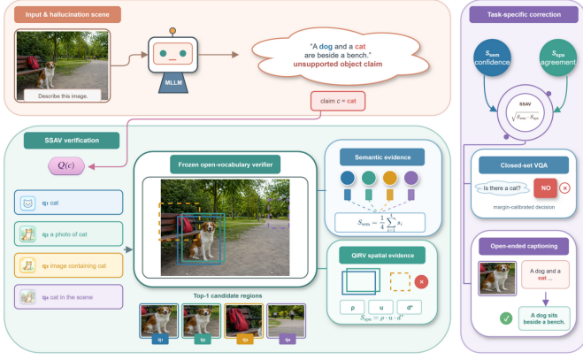
Fig. 1. Overview of Semantic-Spatial Agreement Verification (SSAV). An object claim is extracted from the MLLM response and converted into four semantically equivalent queries. A frozen open-vocabulary verifier returns candidate regions for each query. SSAV combines multi-query semantic support with QIRV spatial evidence, which measures region persistence, spatial overlap, and candidate dominance. The fused evidence calibrates the Yes–No margin in closed-set VQA or filters unsupported object claims in open-ended captioning.
