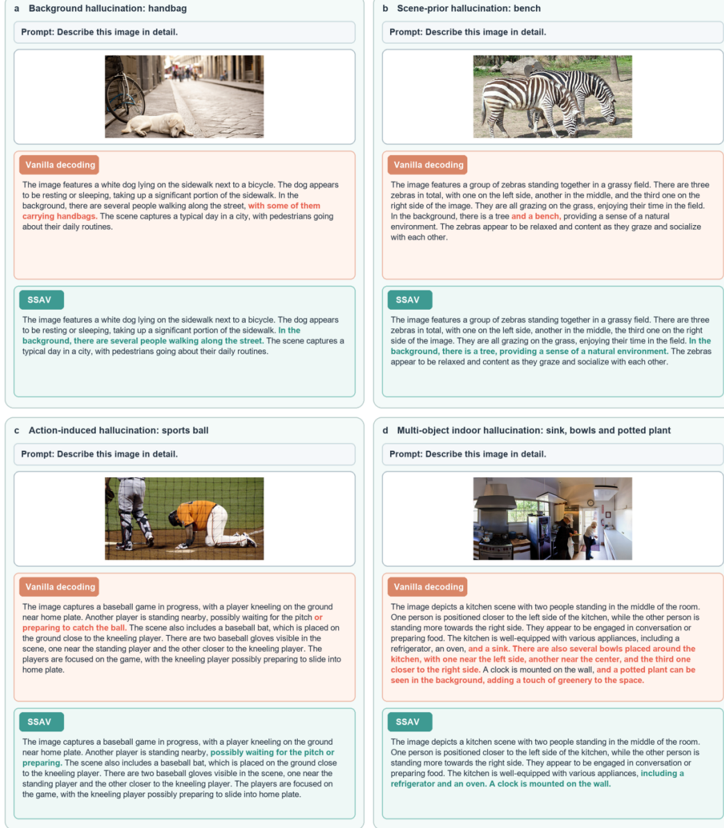
Fig. 4. Qualitative examples of SSAV on CHAIR. Hallucinated claims in the vanilla response are highlighted in red, and descriptions retained after SSAV filtering are highlighted in green. The four cases illustrate background-, scene-prior-, action-induced, and multi-object indoor hallucinations.
