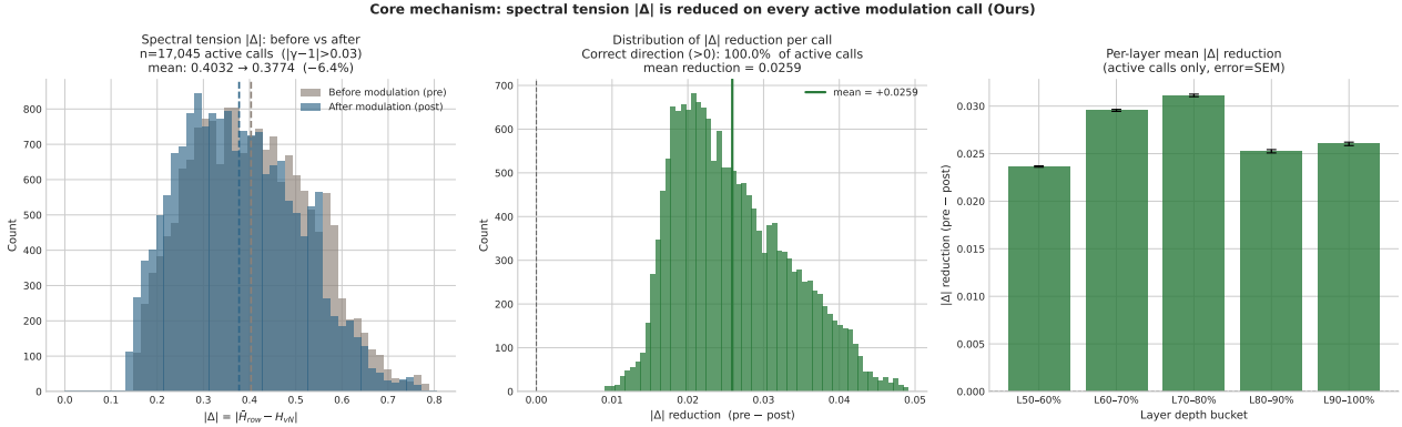
Figure 6. A: Spectral tension |\Delta| before and after modulation on active calls. Left panel : overlaid histograms of pre- and post-modulation |\Delta| . Centre panel : distribution of the per-call reduction |\Delta|_{\text{pre}} - |\Delta|_{\text{post}} . Right panel : mean reduction stratified by layer depth.
