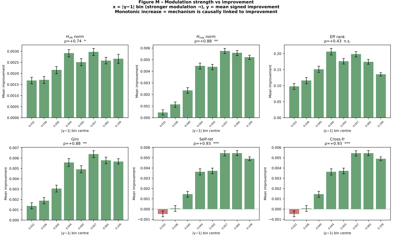
Figure 18. M: Modulation strength vs. mean signed improvement per |\gamma - 1| bin. Active calls are sorted into 8 quantile bins by |\gamma - 1| (stronger modulation rightward). Bars show mean improvement \pm SE. Spearman \rho and significance are annotated.
