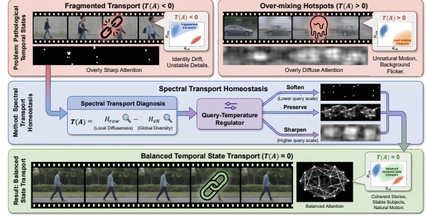
Figure 1. Conceptual view of Temporal State Transport. Good video generation requires temporal attention to stay between two opposite failures: fragmented transport ( T(A) < 0 ) and over-mixing ( T(A) > 0 ). Spectral Tension measures this imbalance by comparing local attention diffuseness with global spectral diversity, while values near zero indicate a more balanced temporal state.
