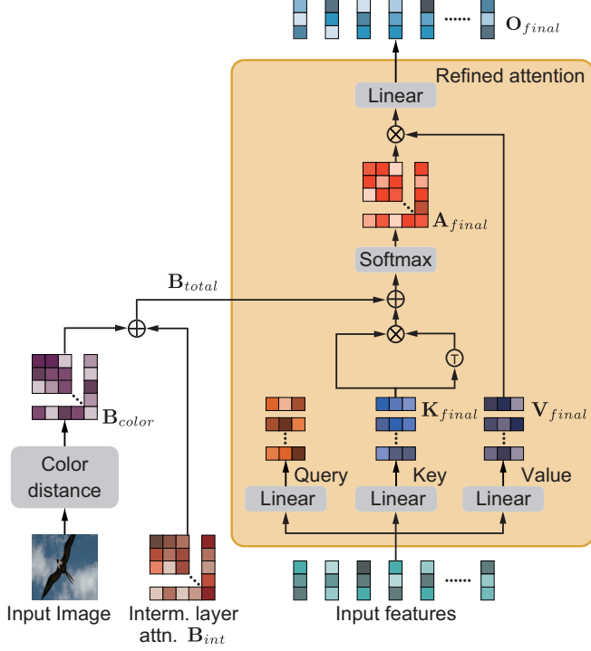
Fig. 2. Details of the proposed refined attention block. Unlike standard self-attention, we employ \mathbf{K}\mathbf{K}^\top similarity instead of \mathbf{Q}\mathbf{K}^\top and inject spatial biases from intermediate layers along with color affinity biases from the input image.
