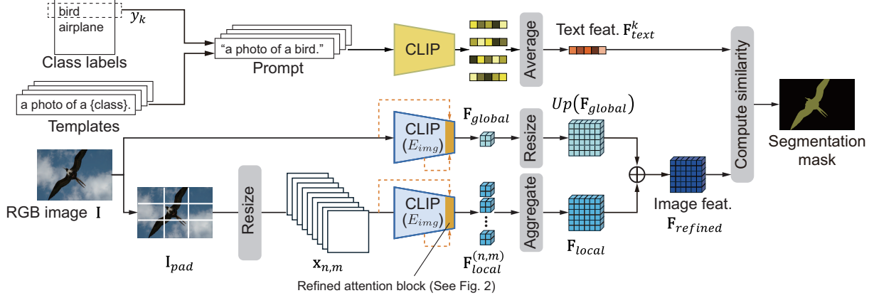
Fig. 1. Overview of MARS-CLIP. Global and local features are fused by a multi-resolution strategy. The final layer (highlighted in orange) injects spatial and color biases to refine boundaries, as detailed in Fig. 2.
