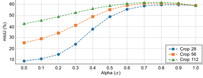
Fig. 3. Impact of fusion weight \alpha across different crop sizes on “V21”.
