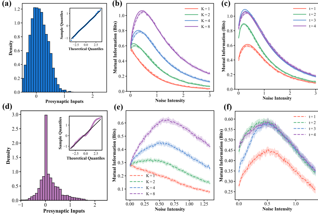
Figure 2: Stochastic resonance behavior of the NGN model characterized by the input-output mutual information MI(I^{t,n-1}, \bar{O}^{t,n}) under the recorded presynaptic Gaussian inputs and non-Gaussian inputs. The Gaussian presynaptic input (a) and the corresponding input-output mutual information versus noise intensity are shown in the first row under different group sizes or iteration: (b) t = 1 ; (c) K = 4 . Here, the theoretical prediction is shown in solid curves and the simulated results are shown in dashed curves. The shaded regions represent one standard deviation of the data. The non-Gaussian input (d) and the corresponding mutual information are shown in the second row under different group sizes or iteration steps: (e) t = 1 ; (f) K = 4 . The initial noise intensity for training ResNet-18 is \sigma_0 = 0.5 . The quantile-quantile (Q-Q) plot embedded in (a) and (d) signifies how the presynaptic input deviates from Gaussian distribution. The non-monotonic curves in (b), (c), (e) and (f) manifest the occurrence of stochastic resonance.
