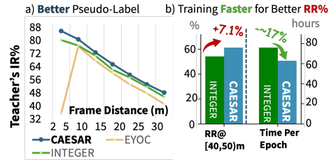
Fig. 2: Performance: Our method leverages this native ability to improve unsupervised point cloud registration even with reduced training time (Sec. 4.3).
