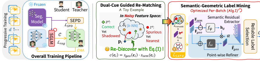
Fig. 3: Overall Pipeline. DCRM recovers correct correspondences obscured by feature-space noise by jointly considering geometric saliency and semantic similarity. The train-only SGLM refines the teacher’s feature space and mines high-quality pseudo-labels. The student is trained with its original registration loss on \mathcal{C} and the SPD objective to strengthen semantic awareness.
