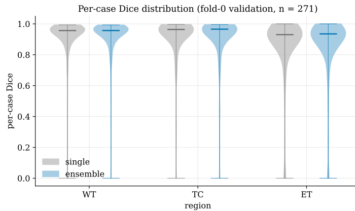
Fig. 1. Per-case Dice distributions on the internal validation split ( n = 271 ), split-0 single model vs 3-seed deep ensemble, by region. The mass concentrates near 1.0 with thin tails reaching 0, so the typical case is excellent and the mean is set by a hard-case tail.
